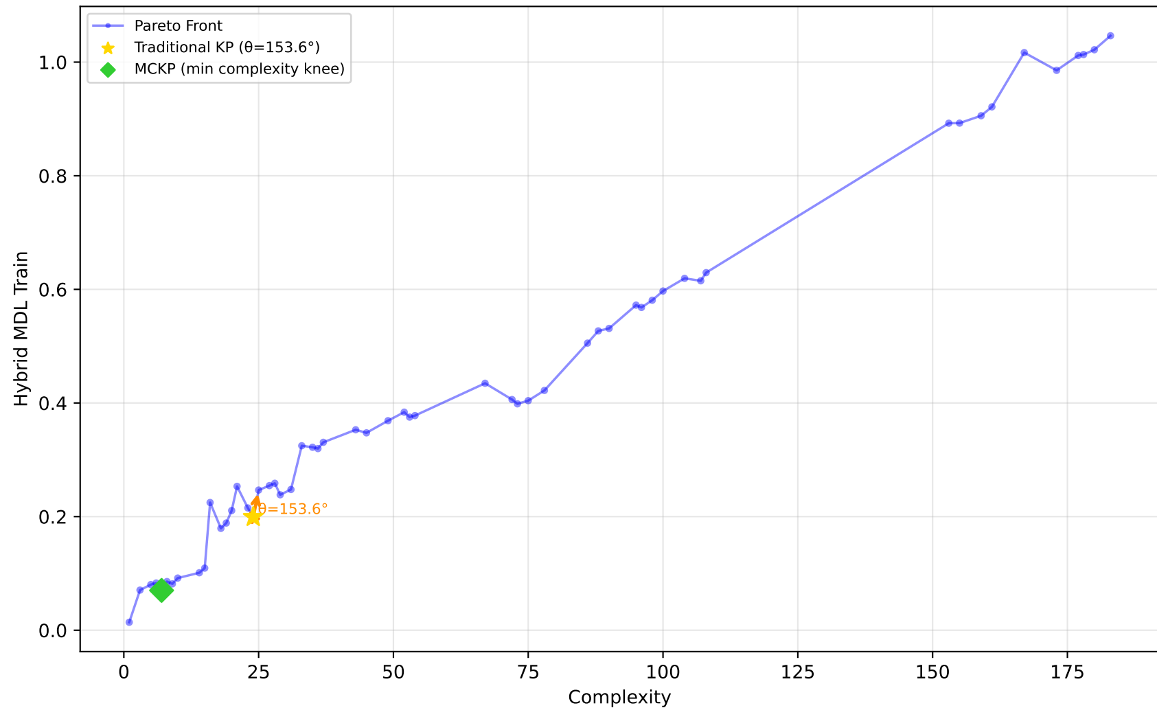
192_vineyard - Run 17 - MVP - Hybrid MDL Train \lambda_1=0.40, \lambda_2=0.00, \lambda_3=1.00 | Difficulty: 0.71 | Method: hmr
