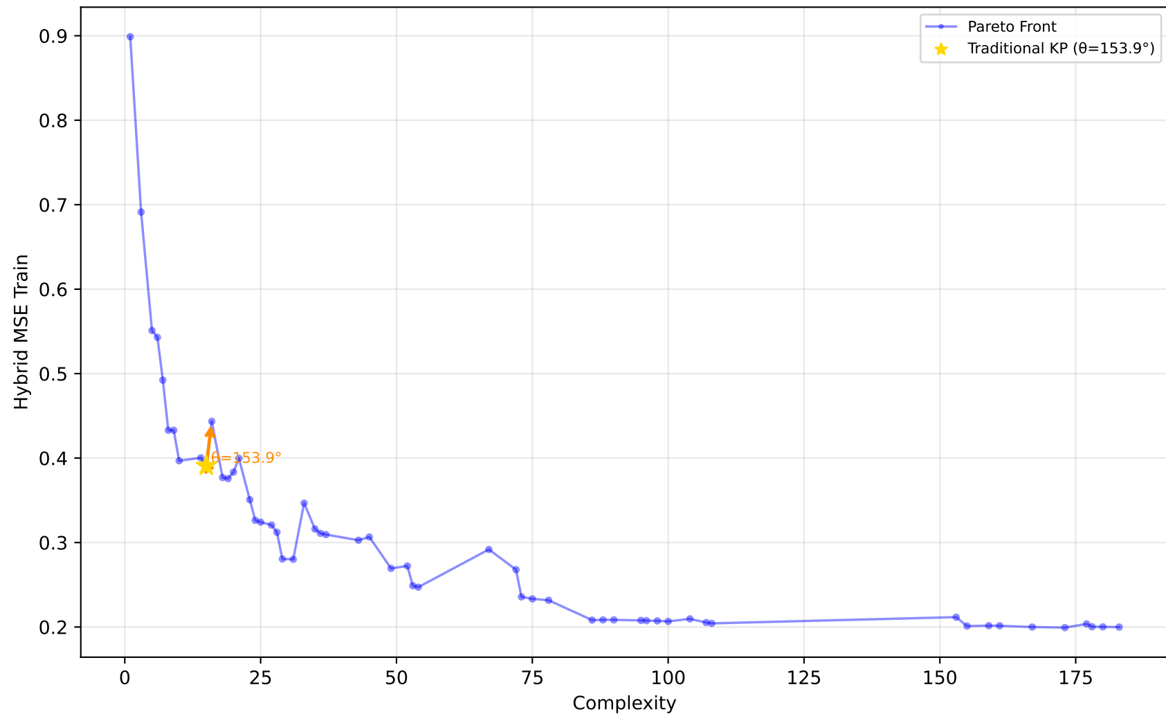
192_vineyard - Run 17 - MVP - Hybrid MSE Train \lambda_1=0.40, \lambda_2=0.00, \lambda_3=1.00 | Difficulty: 0.71 | Method: hmr
