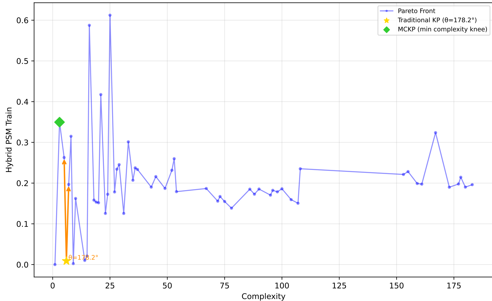
192_vineyard - Run 17 - MVP - Hybrid PSM Train \lambda_1=0.00, \lambda_2=0.30, \lambda_3=1.00 | Difficulty: 0.71 | Method: hmr
