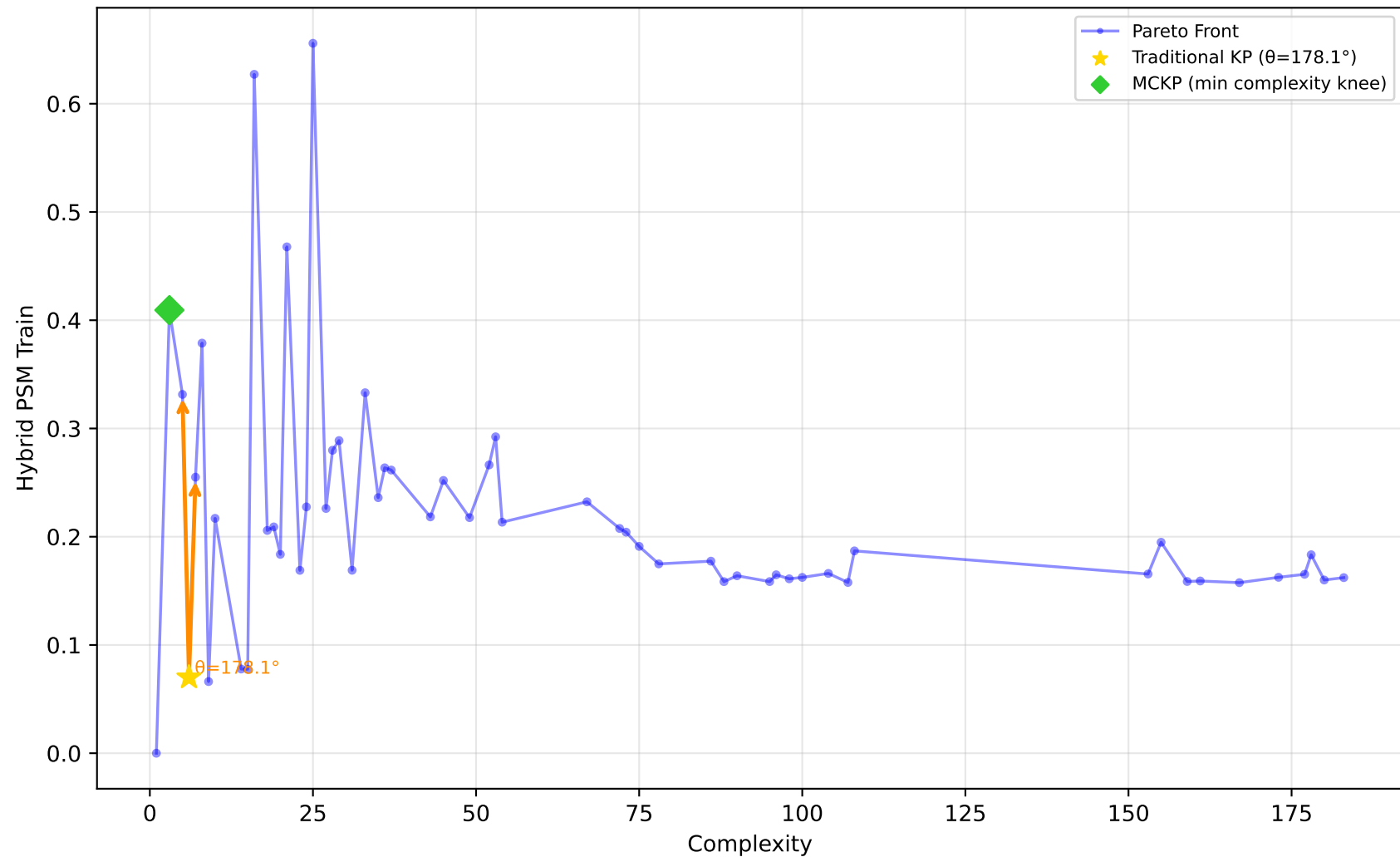
192_vineyard - Run 17 - MVP - Hybrid PSM Train \lambda_1=0.40, \lambda_2=0.00, \lambda_3=1.00 | Difficulty: 0.71 | Method: hmr
