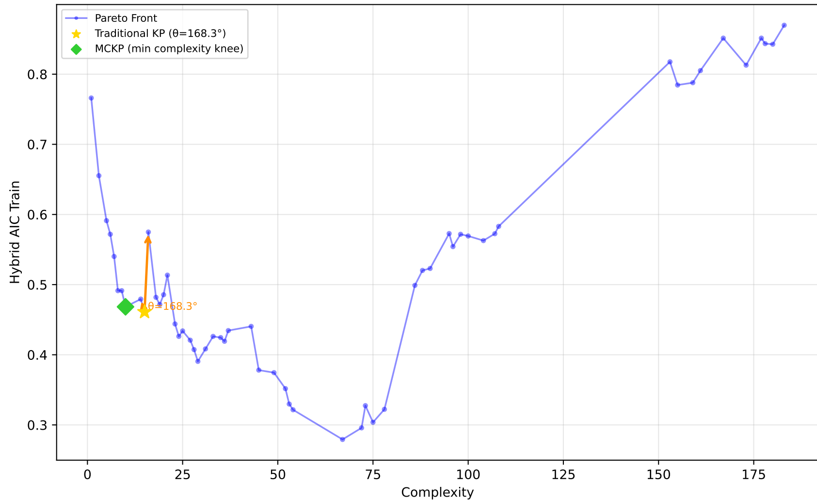
192_vineyard - Run 17 - SVP - Hybrid AIC Train \lambda_1=0.00, \bar{\lambda}_2=1.00, \lambda_3=1.00 | Difficulty: 0.71 | Method: hmr
