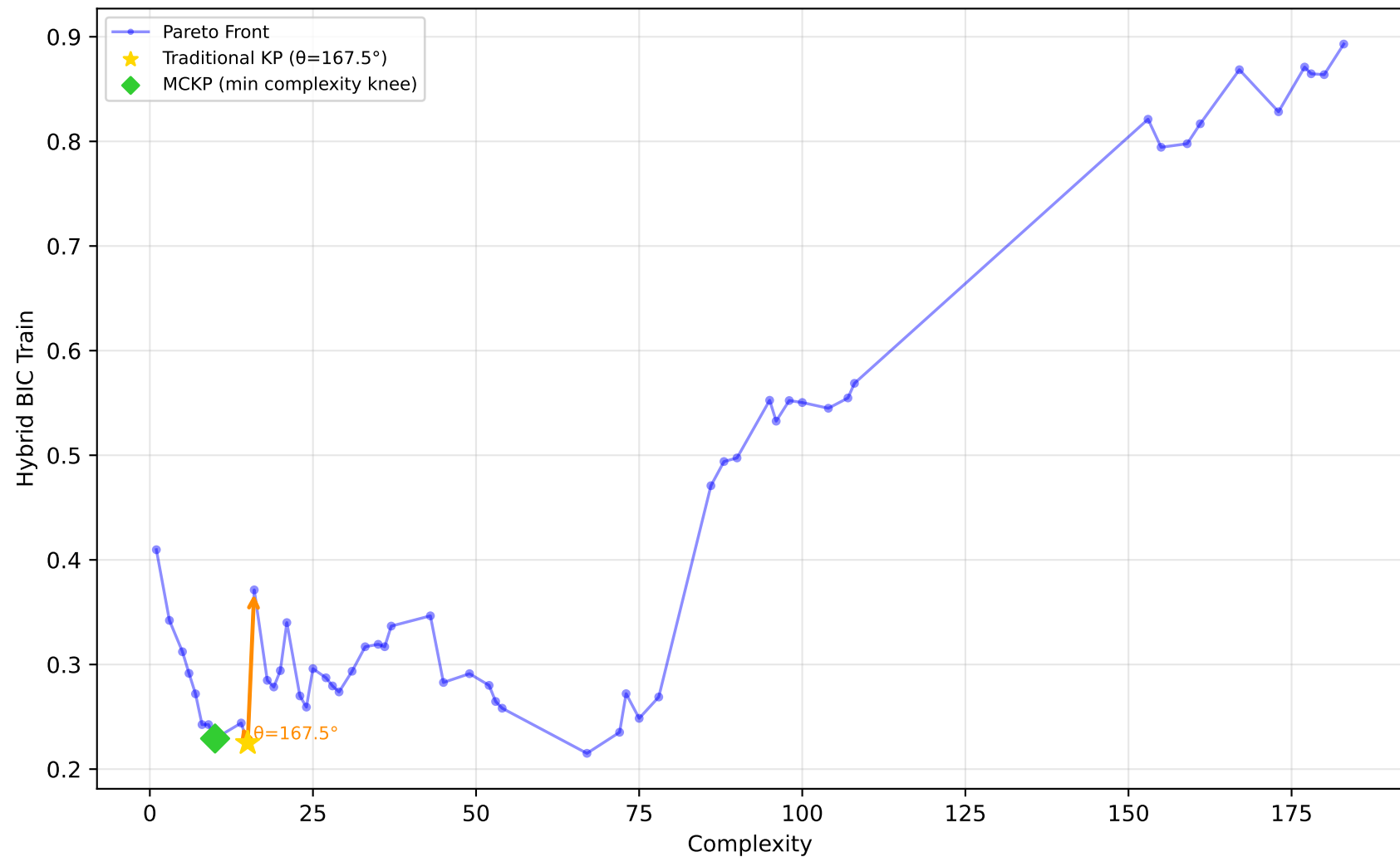
192_vineyard - Run 17 - SVP - Hybrid BIC Train \lambda_1=0.00, \bar{\lambda}_2=1.00, \lambda_3=1.00 | Difficulty: 0.71 | Method: hmr
