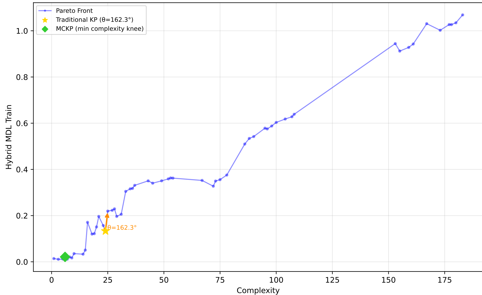
192_vineyard - Run 17 - SVP - Hybrid MDL Train \lambda_1=0.00, \lambda_2=1.00, \lambda_3=1.00 | Difficulty: 0.71 | Method: hmr
