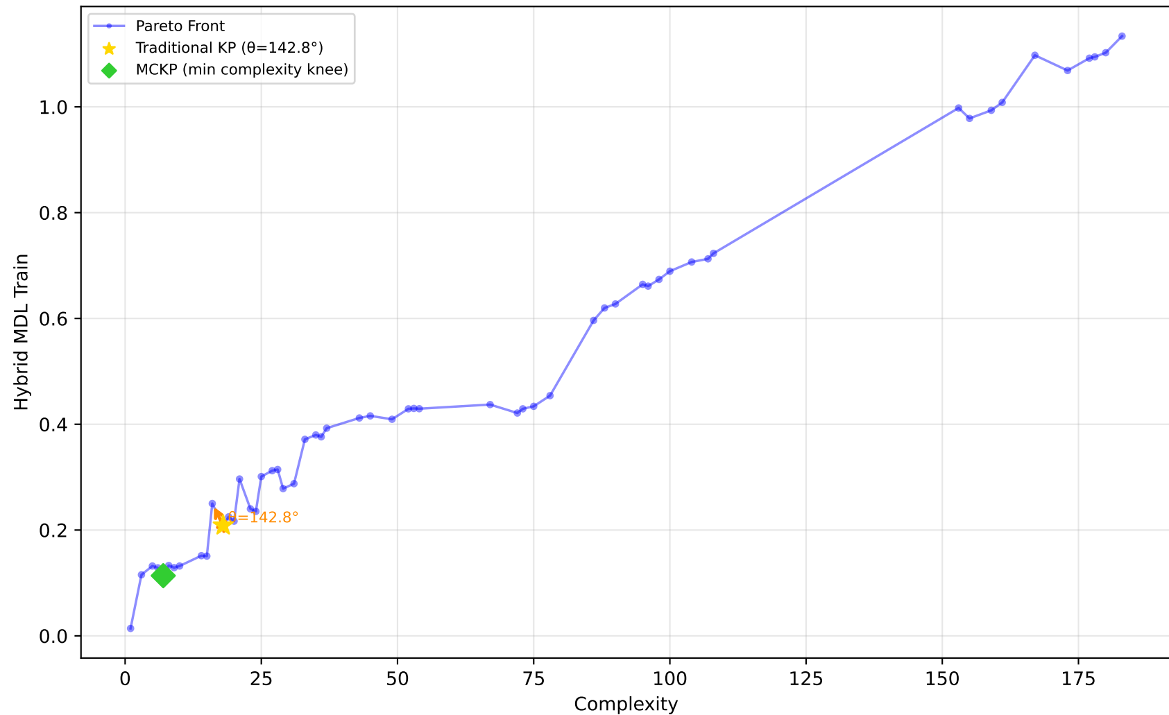
192_vineyard - Run 17 - SVP - Hybrid MDL Train \lambda_1=0.70, \bar{\lambda}_2=0.70, \lambda_3=0.90 | Difficulty: 0.71 | Method: hmr
