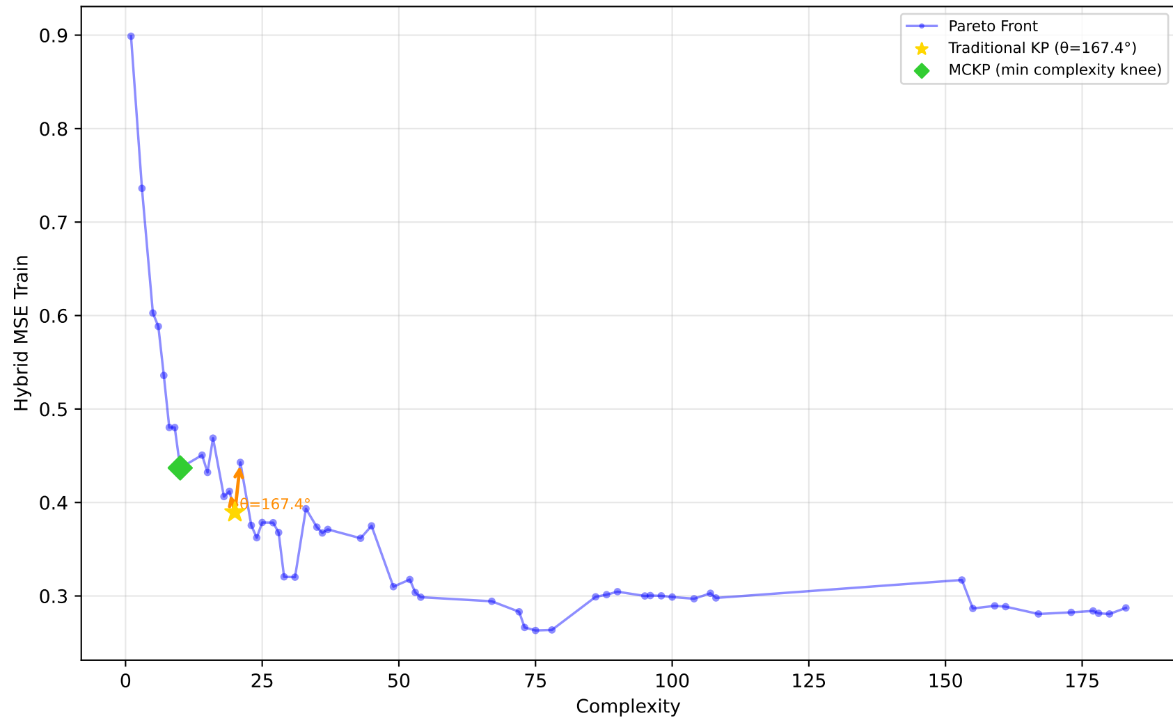
192_vineyard - Run 17 - SVP - Hybrid MSE Train \lambda_1=0.70, \bar{\lambda}_2=0.70, \lambda_3=0.90 | Difficulty: 0.71 | Method: hmr
