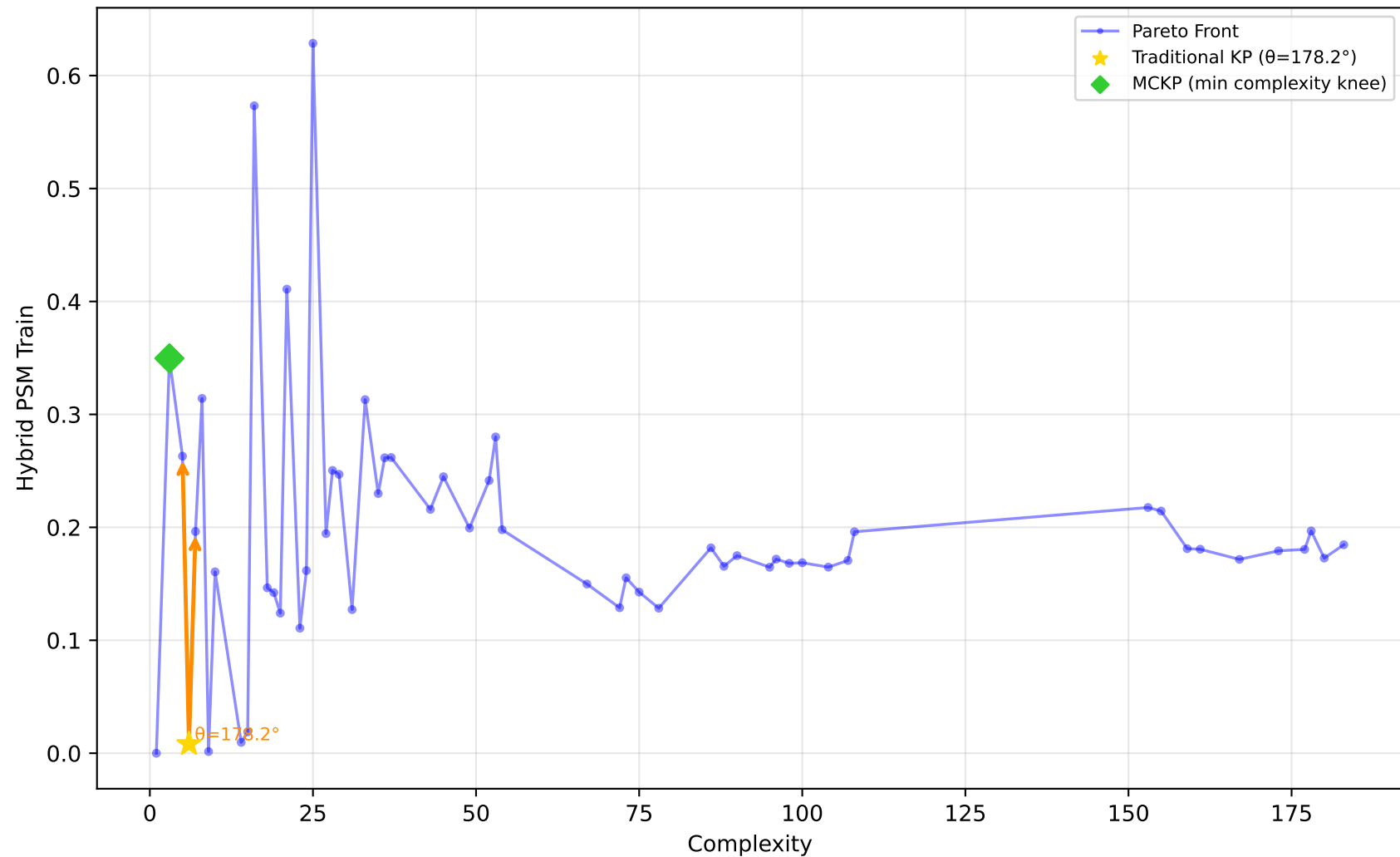
192_vineyard - Run 17 - SVP - Hybrid PSM Train \lambda_1=0.00, \bar{\lambda}_2=1.00, \lambda_3=1.00 | Difficulty: 0.71 | Method: hmr
