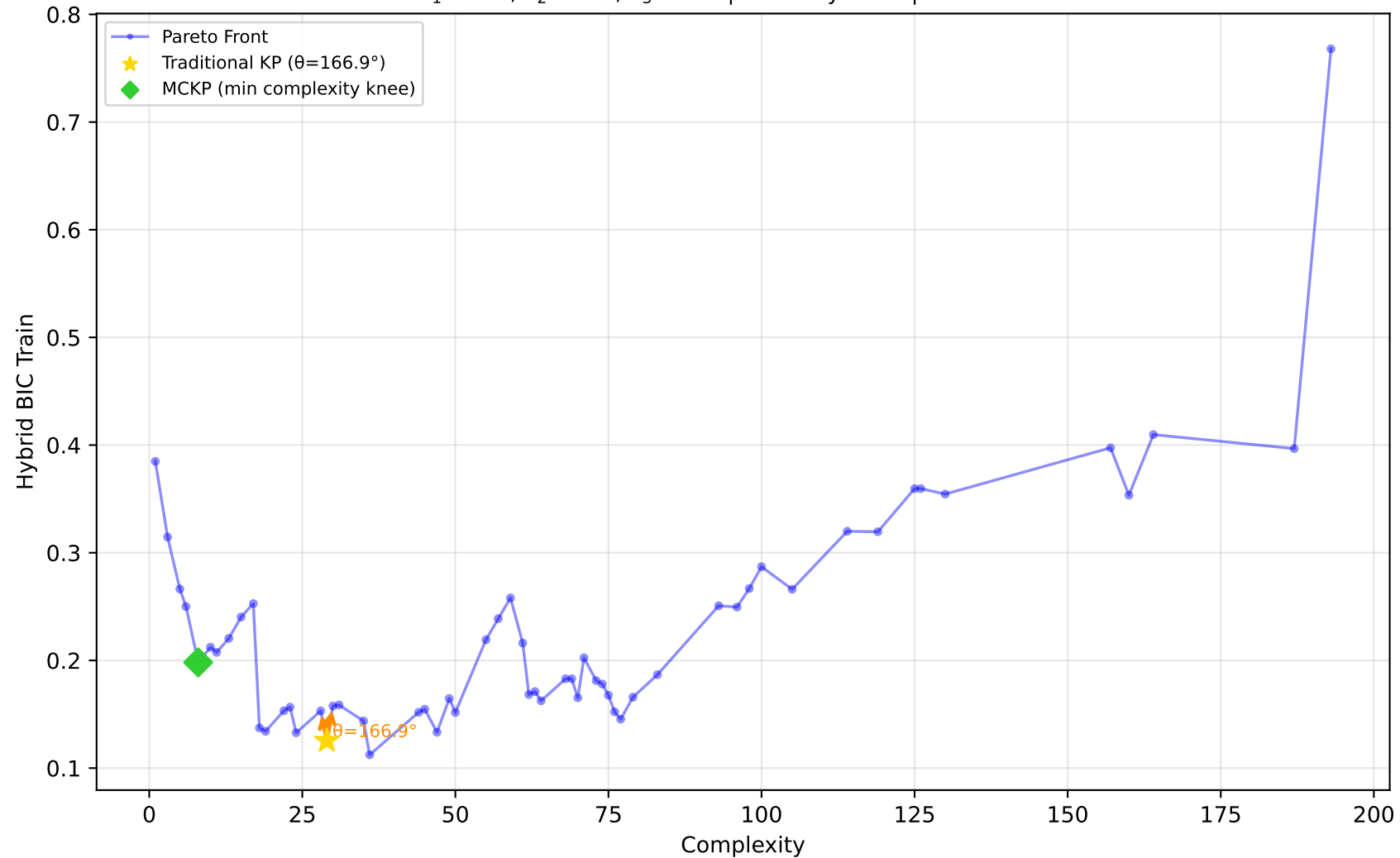
192_vineyard - Run 18 - MVP - Hybrid BIC Train \lambda_1=0.00, \lambda_2=0.30, \lambda_3=1.00 | Difficulty: 1.00 | Method: hmr
