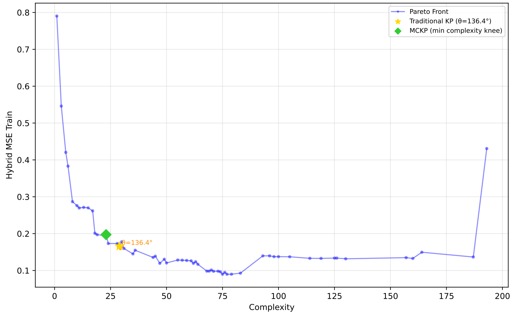
192_vineyard - Run 18 - MVP - Hybrid MSE Train \lambda_1=0.00, \bar{\lambda}_2=0.30, \lambda_3=1.00 | Difficulty: 1.00 | Method: hmr
