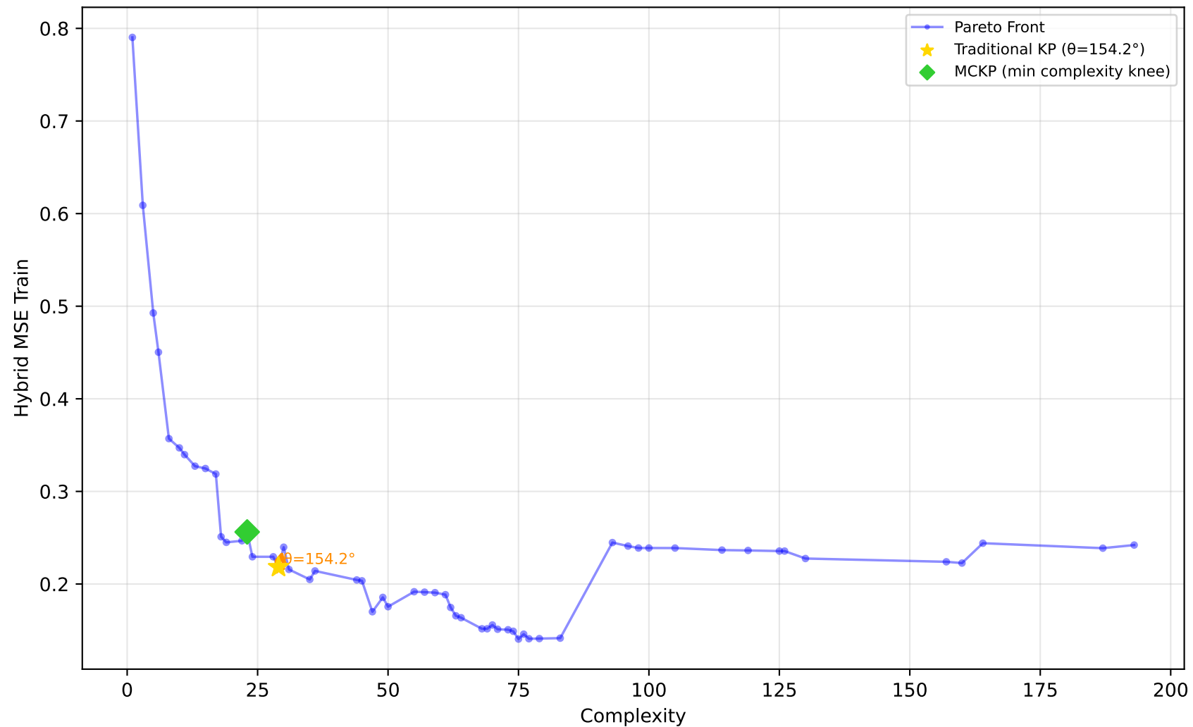
192_vineyard - Run 18 - MVP - Hybrid MSE Train \lambda_1=0.40, \bar{\lambda}_2=0.00, \lambda_3=1.00 | Difficulty: 1.00 | Method: hmr
