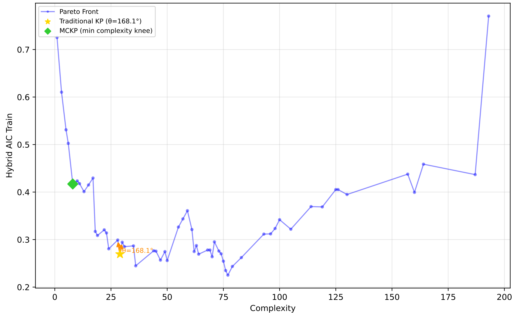
192_vineyard - Run 18 - SVP - Hybrid AIC Train \lambda_1=0.00, \bar{\lambda}_2=1.00, \lambda_3=1.00 | Difficulty: 1.00 | Method: hmr
