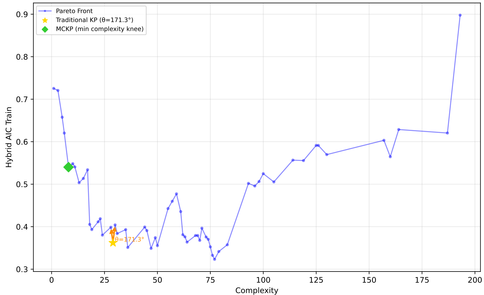
192_vineyard - Run 18 - SVP - Hybrid AIC Train \lambda_1=0.70, \bar{\lambda}_2=0.70, \lambda_3=0.90 | Difficulty: 1.00 | Method: hmr
