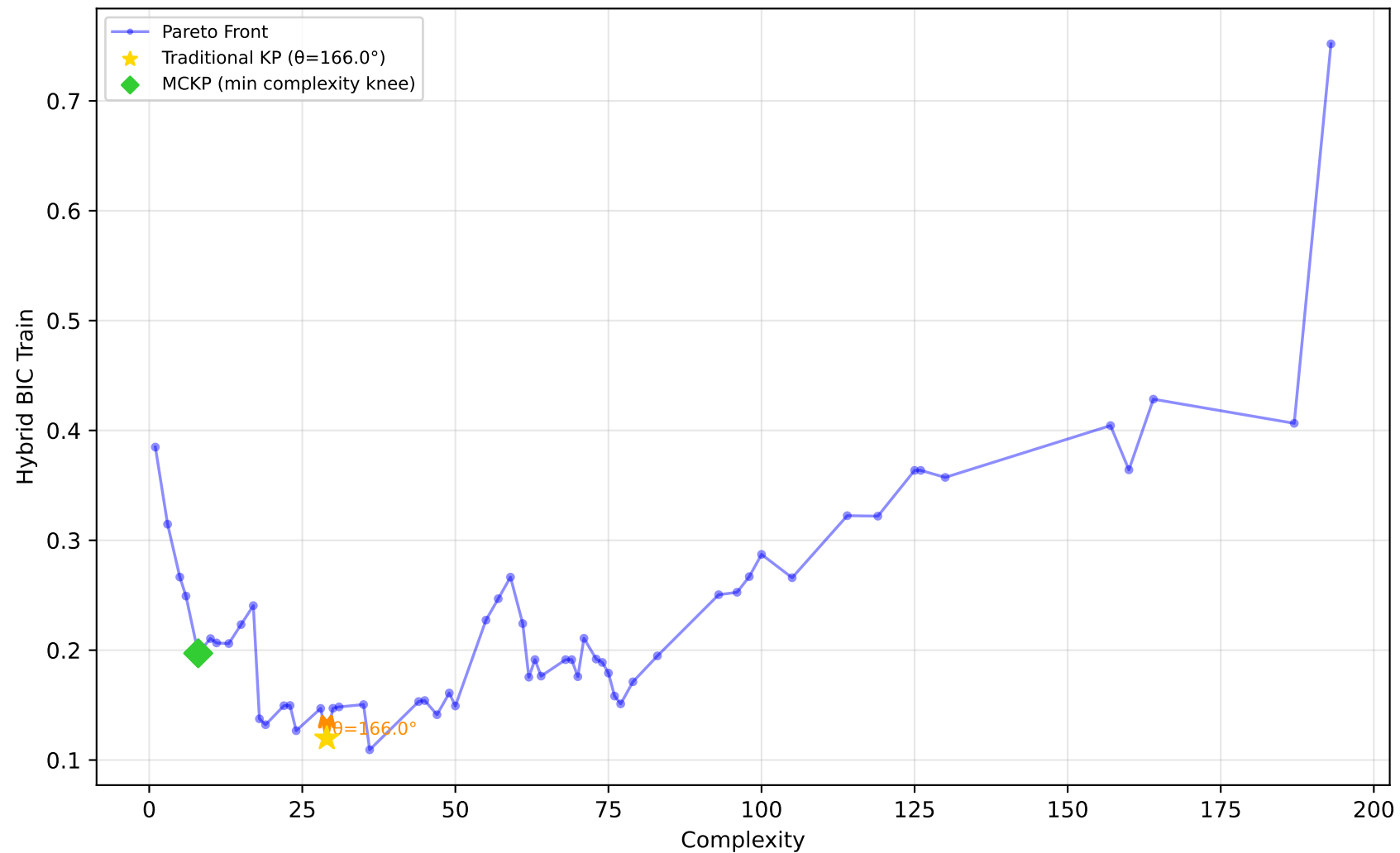
192_vineyard - Run 18 - SVP - Hybrid BIC Train \lambda_1=0.00, \bar{\lambda}_2=1.00, \lambda_3=1.00 | Difficulty: 1.00 | Method: hmr
