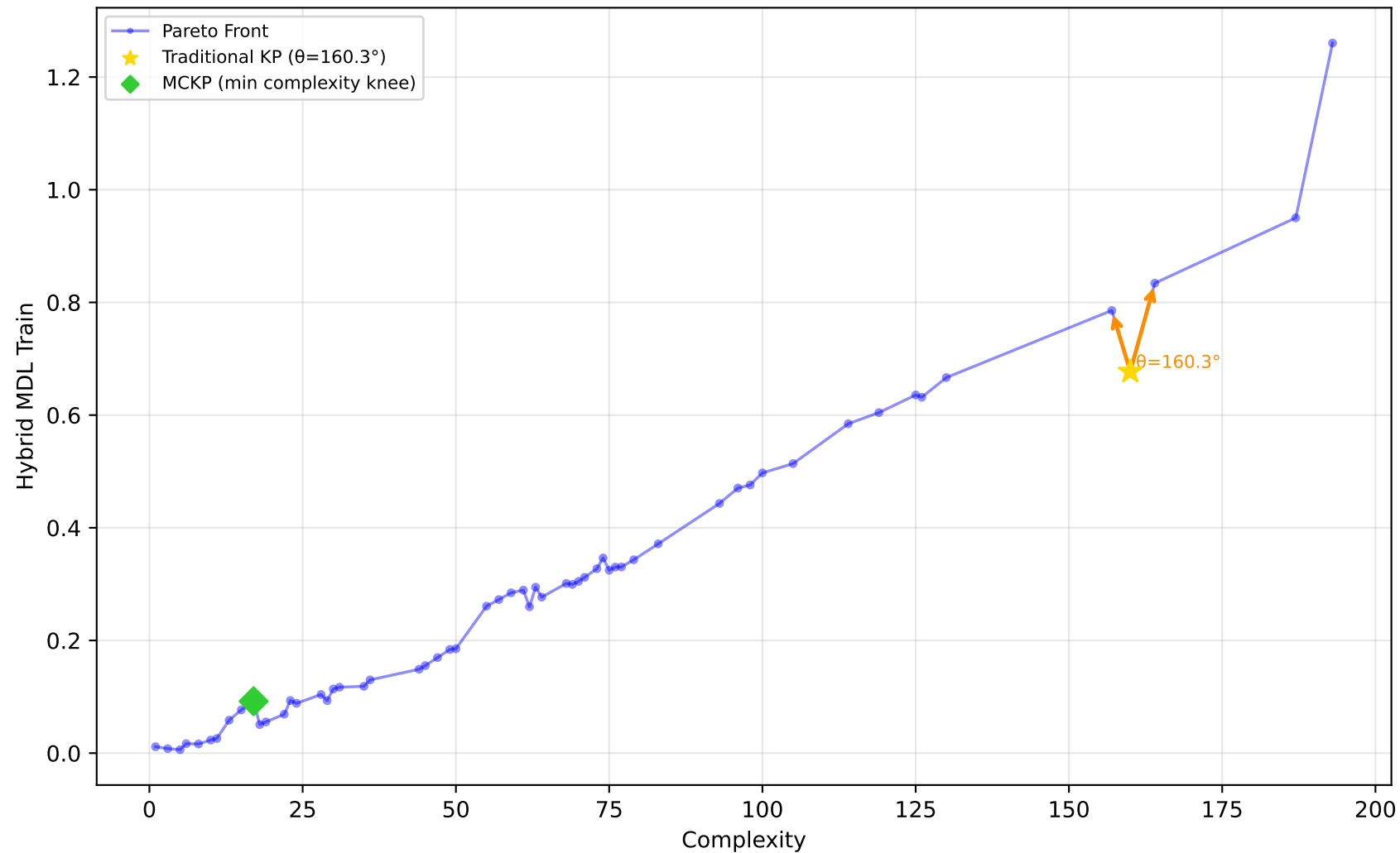
192_vineyard - Run 18 - SVP - Hybrid MDL Train \lambda_1=0.00, \bar{\lambda}_2=1.00, \lambda_3=1.00 | Difficulty: 1.00 | Method: hmr
