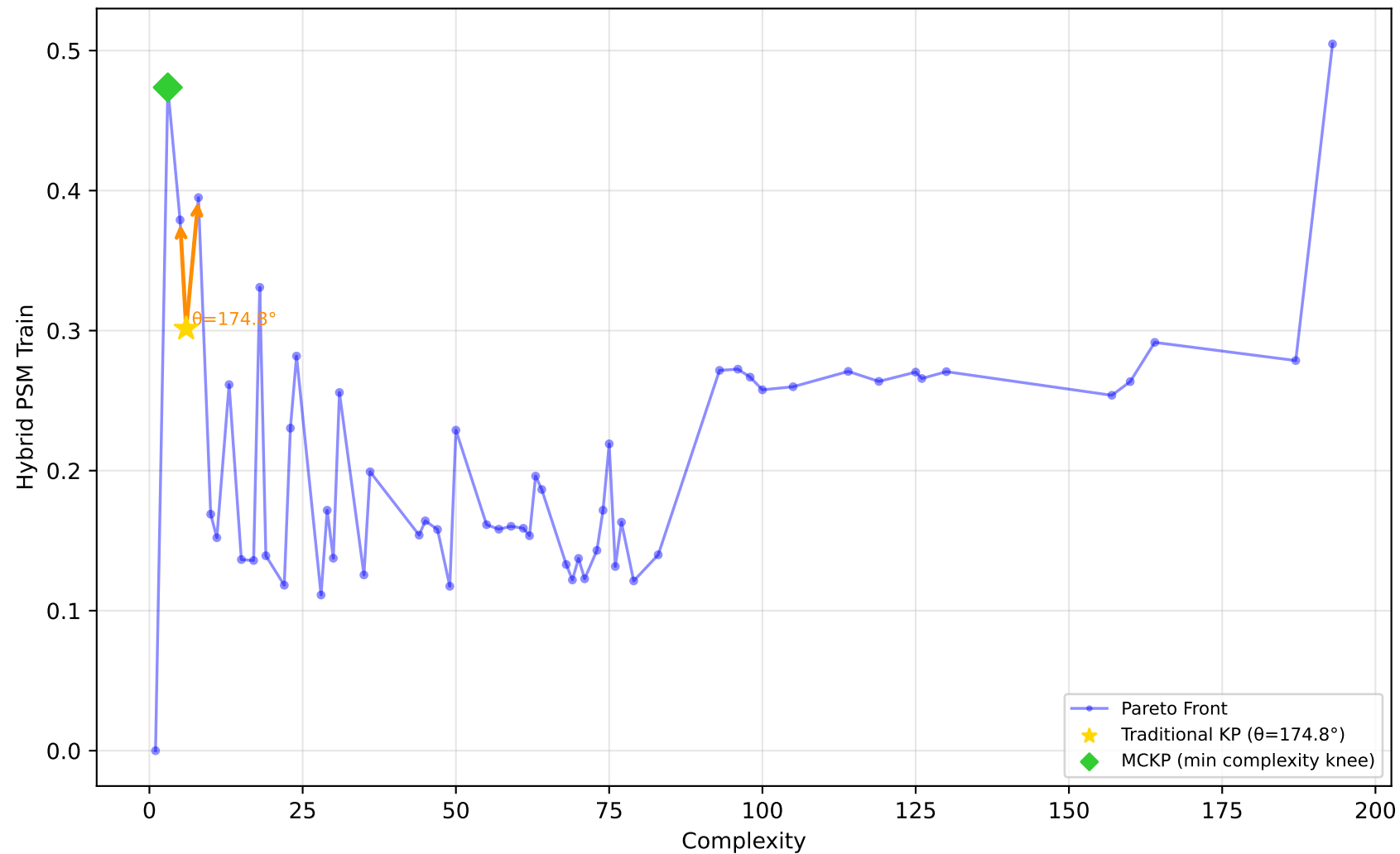
192_vineyard - Run 18 - SVP - Hybrid PSM Train \lambda_1=0.70, \lambda_2=0.70, \lambda_3=0.90 | Difficulty: 1.00 | Method: hmr
