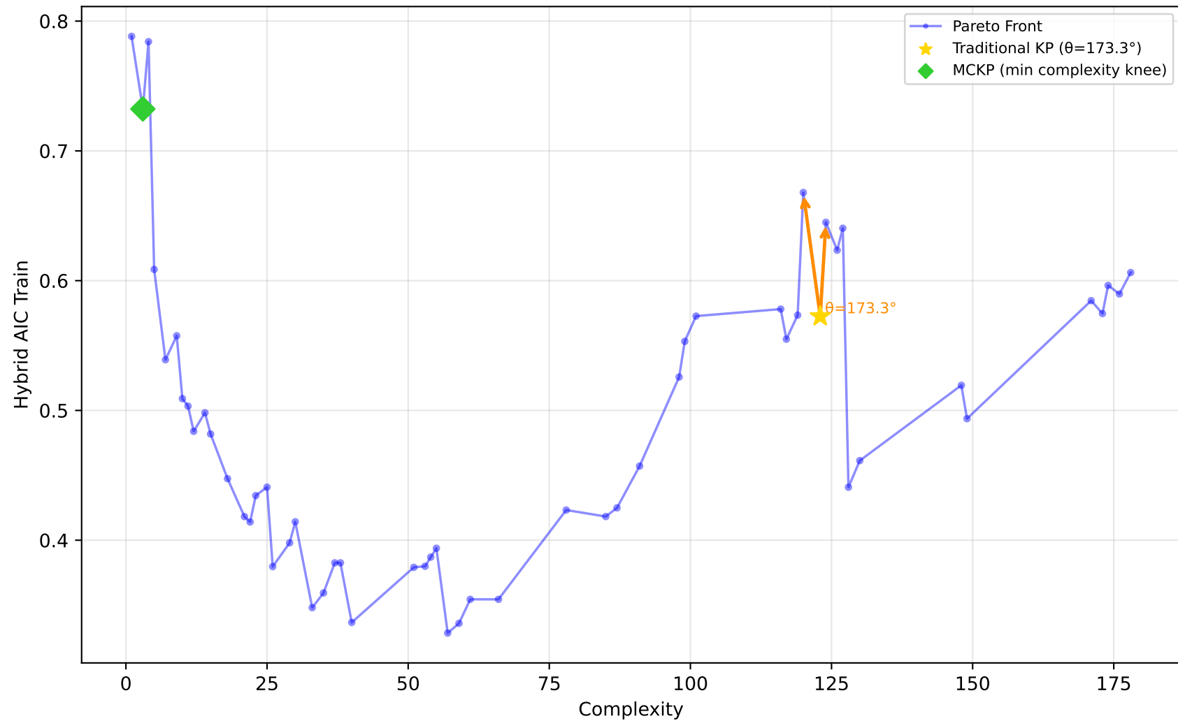
192_vineyard - Run 19 - MVP - Hybrid AIC Train \lambda_1=0.40, \bar{\lambda}_2=0.00, \lambda_3=1.00 | Difficulty: 0.89 | Method: hmr
