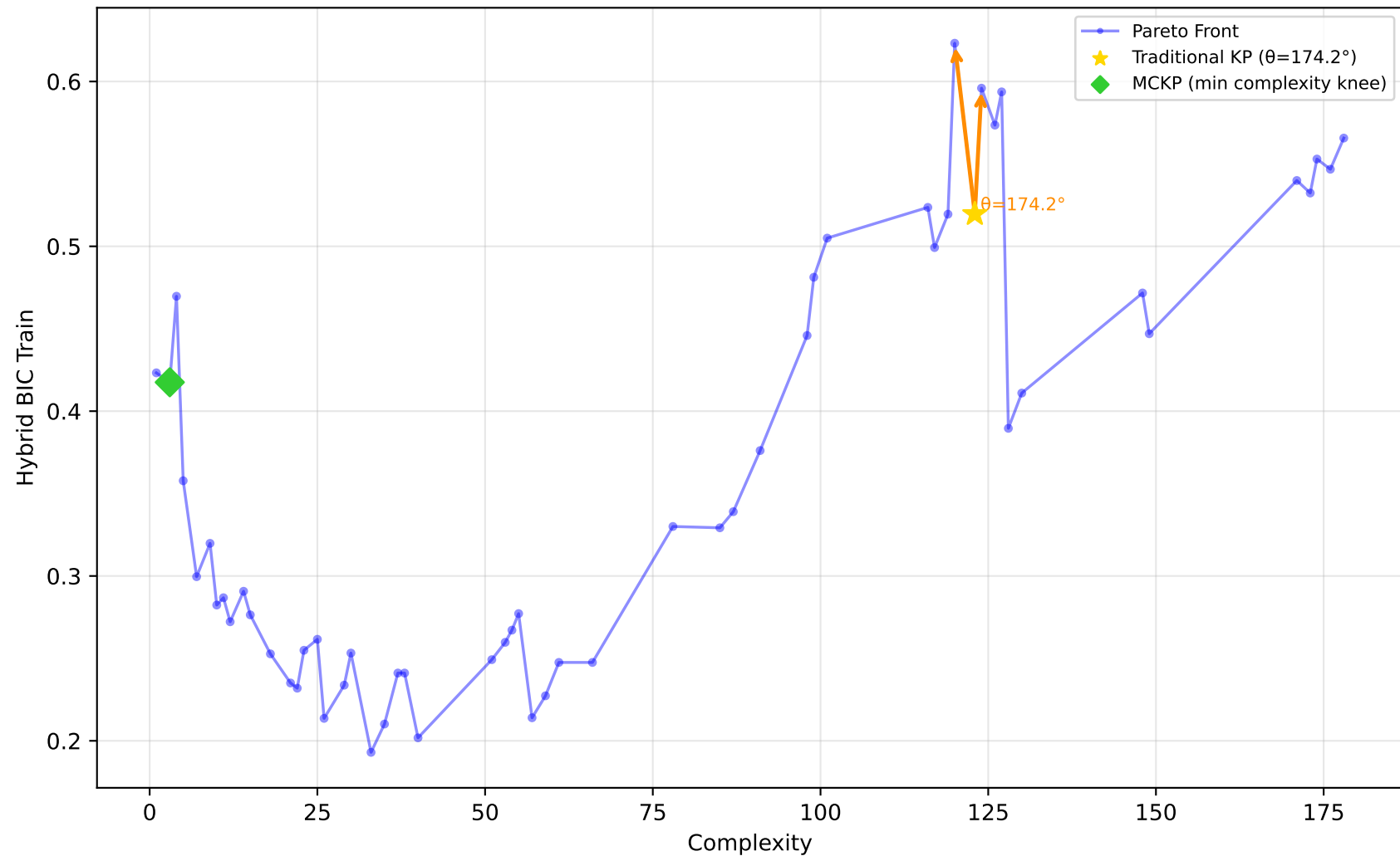
192_vineyard - Run 19 - MVP - Hybrid BIC Train \lambda_1=0.40, \bar{\lambda}_2=0.00, \lambda_3=1.00 | Difficulty: 0.89 | Method: hmr
