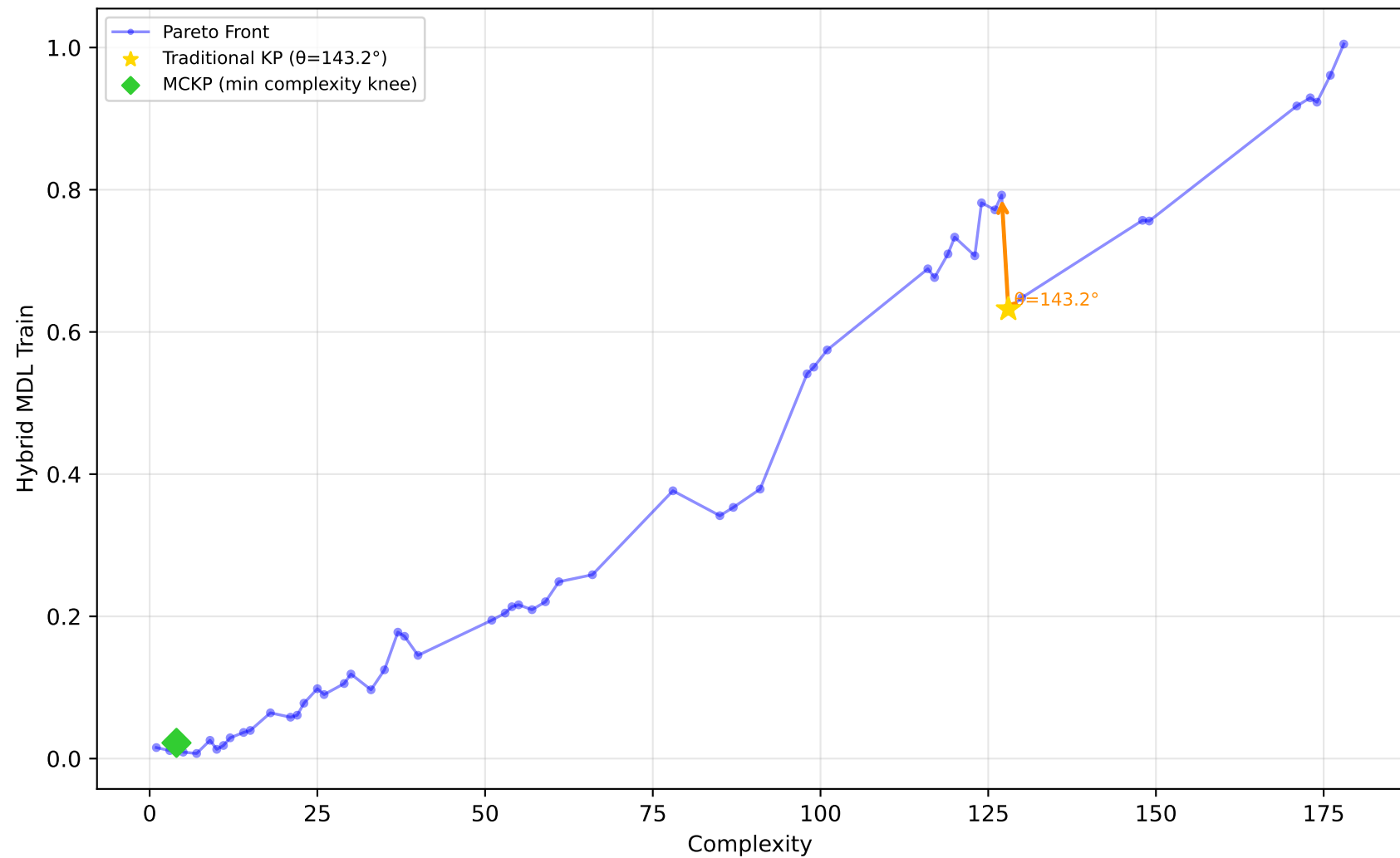
192_vineyard - Run 19 - MVP - Hybrid MDL Train \lambda_1=0.00, \lambda_2=0.30, \lambda_3=1.00 | Difficulty: 0.89 | Method: hmr
