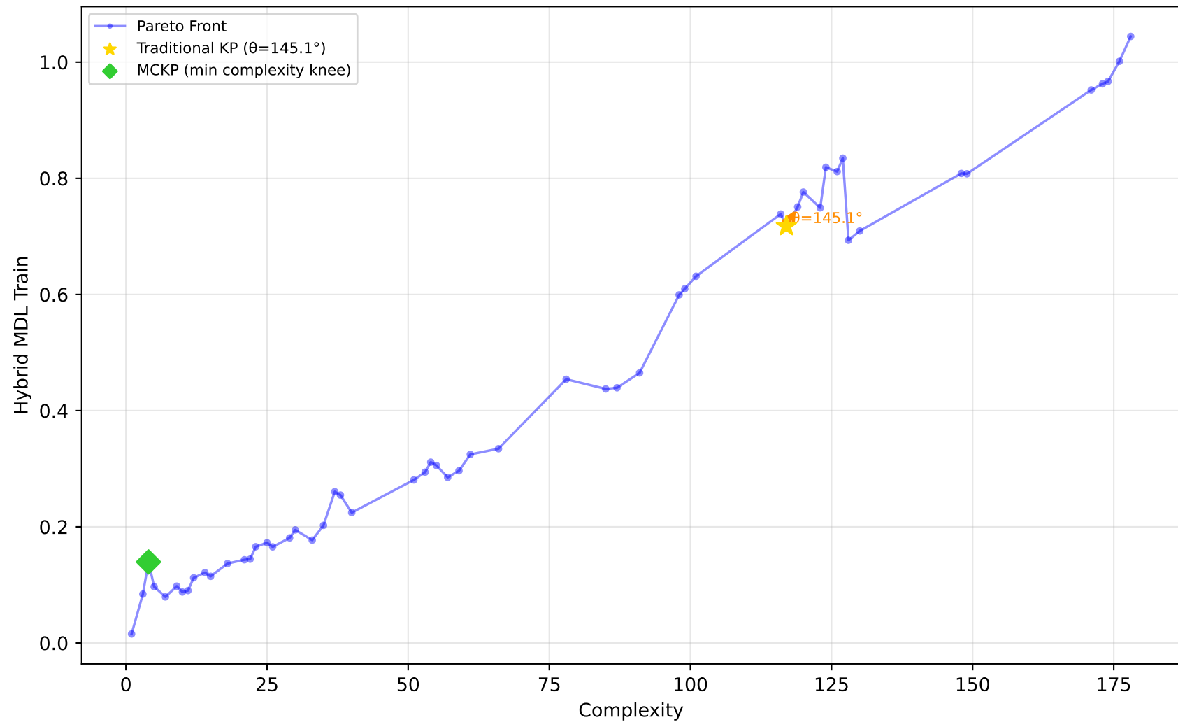
192_vineyard - Run 19 - MVP - Hybrid MDL Train \lambda_1=0.40, \lambda_2=0.00, \lambda_3=1.00 | Difficulty: 0.89 | Method: hmr
