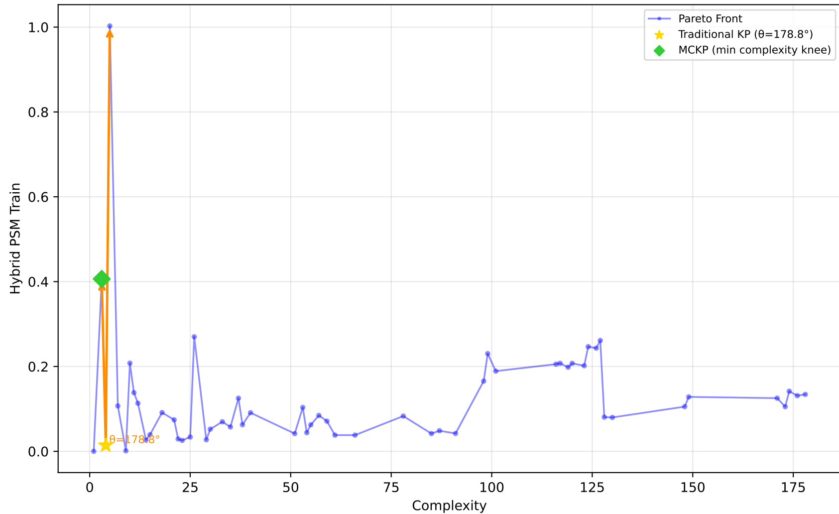
192_vineyard - Run 19 - MVP - Hybrid PSM Train \lambda_1=0.00, \lambda_2=0.30, \lambda_3=1.00 | Difficulty: 0.89 | Method: hmr
