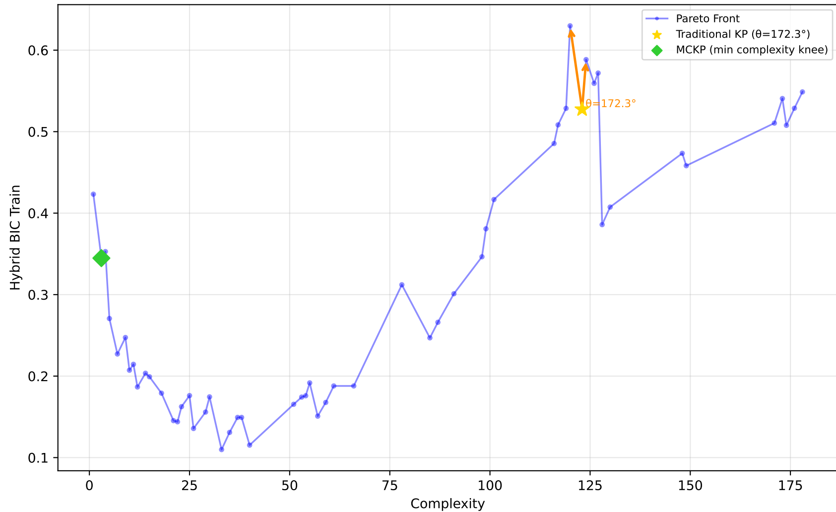
192_vineyard - Run 19 - SVP - Hybrid BIC Train \lambda_1=0.00, \bar{\lambda}_2=1.00, \lambda_3=1.00 | Difficulty: 0.89 | Method: hmr
