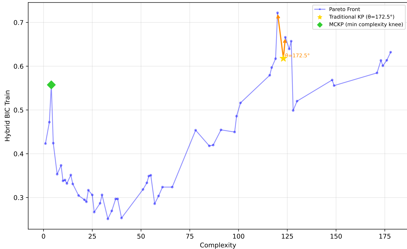
192_vineyard - Run 19 - SVP - Hybrid BIC Train \lambda_1=0.70, \bar{\lambda}_2=0.70, \lambda_3=0.90 | Difficulty: 0.89 | Method: hmr
