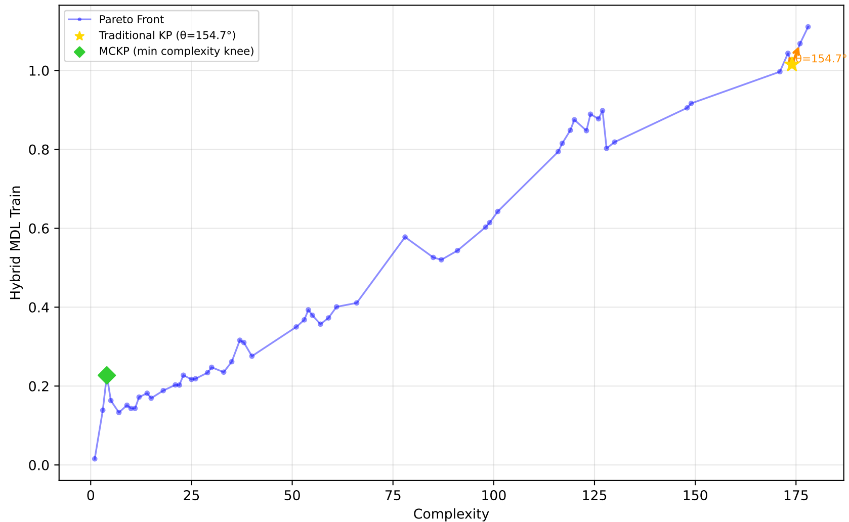
192_vineyard - Run 19 - SVP - Hybrid MDL Train \lambda_1=0.70, \bar{\lambda}_2=0.70, \lambda_3=0.90 | Difficulty: 0.89 | Method: hmr
