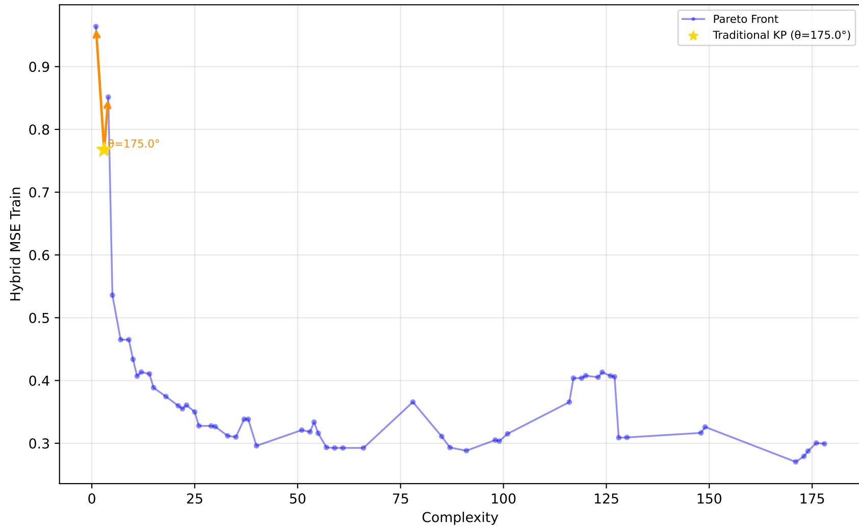
192_vineyard - Run 19 - SVP - Hybrid MSE Train \lambda_1=0.70, \bar{\lambda}_2=0.70, \lambda_3=0.90 | Difficulty: 0.89 | Method: hmr
