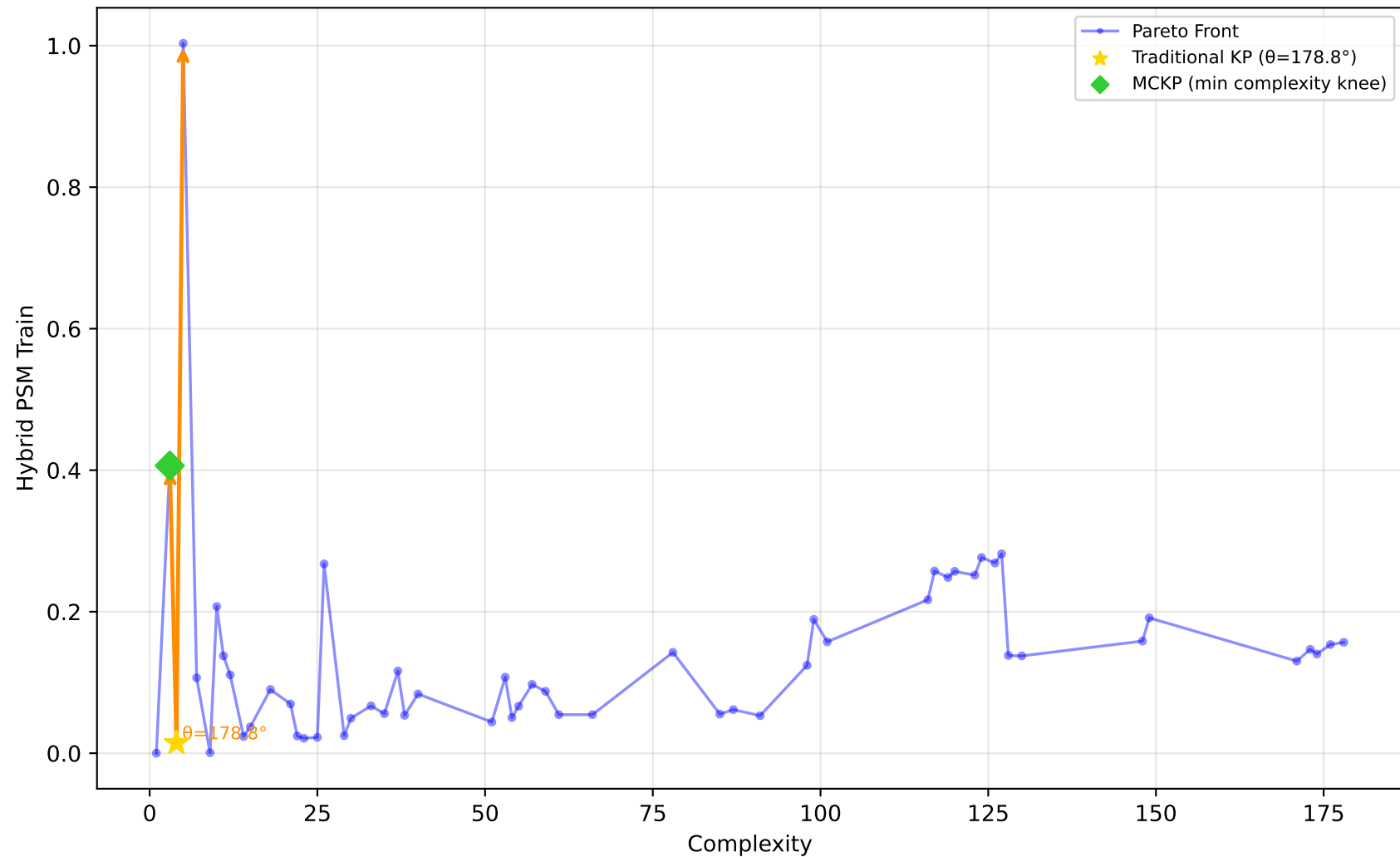
192_vineyard - Run 19 - SVP - Hybrid PSM Train \lambda_1=0.00, \bar{\lambda}_2=1.00, \lambda_3=1.00 | Difficulty: 0.89 | Method: hmr
