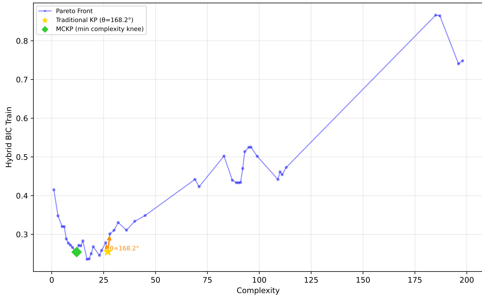
192_vineyard - Run 1 - MVP - Hybrid BIC Train \lambda_1=0.00, \lambda_2=0.30, \lambda_3=1.00 | Difficulty: 0.27 | Method: mckp
