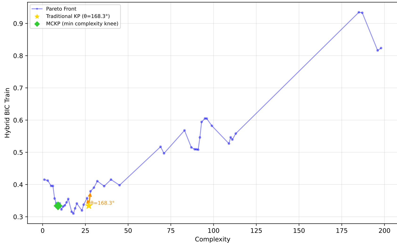
192_vineyard - Run 1 - MVP - Hybrid BIC Train \lambda_1=0.40, \lambda_2=0.00, \lambda_3=1.00 | Difficulty: 0.27 | Method: mckp
