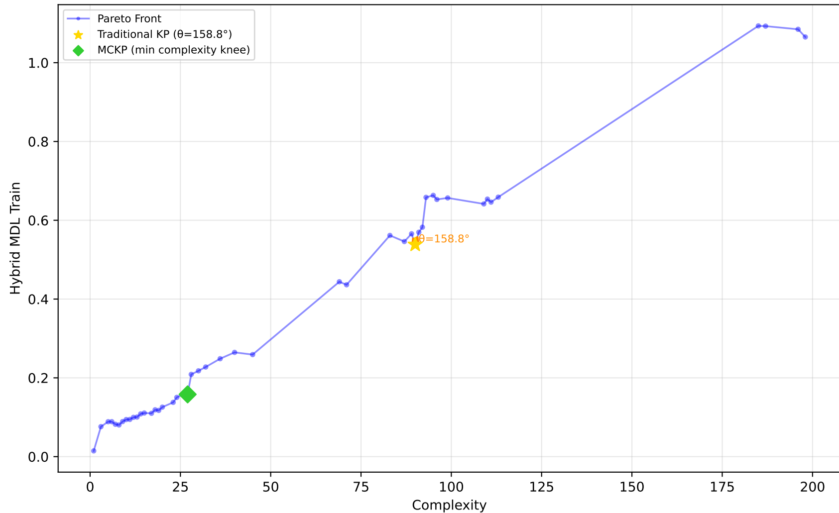
192_vineyard - Run 1 - MVP - Hybrid MDL Train \lambda_1=0.40, \lambda_2=0.00, \lambda_3=1.00 | Difficulty: 0.27 | Method: mckp
