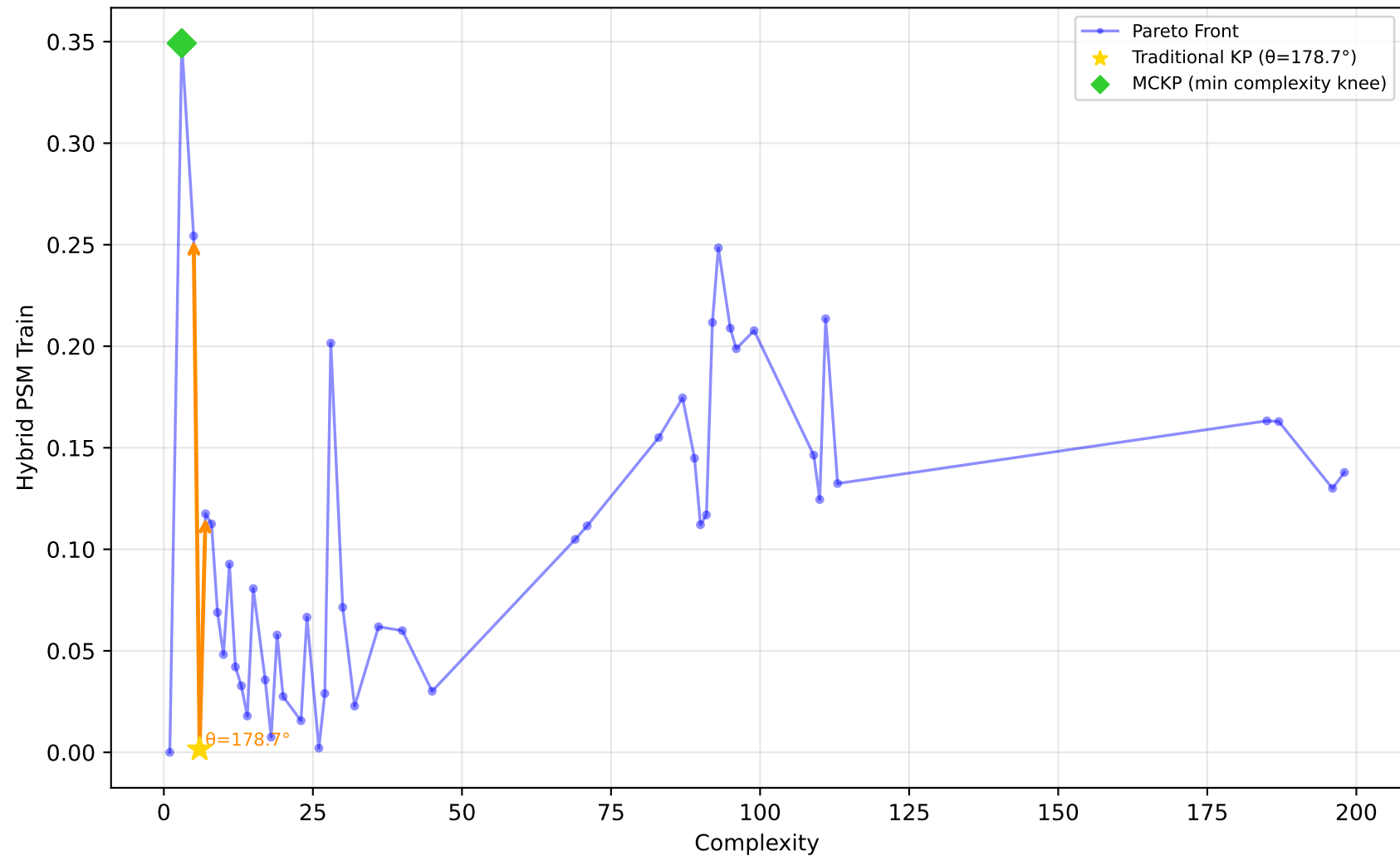
192_vineyard - Run 1 - MVP - Hybrid PSM Train \lambda_1=0.00, \lambda_2=0.30, \lambda_3=1.00 | Difficulty: 0.27 | Method: mckp
