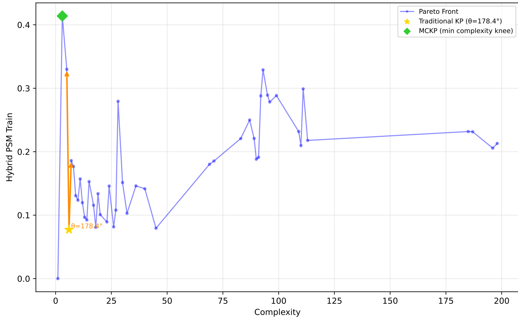
192_vineyard - Run 1 - MVP - Hybrid PSM Train \lambda_1=0.40, \lambda_2=0.00, \lambda_3=1.00 | Difficulty: 0.27 | Method: mckp
