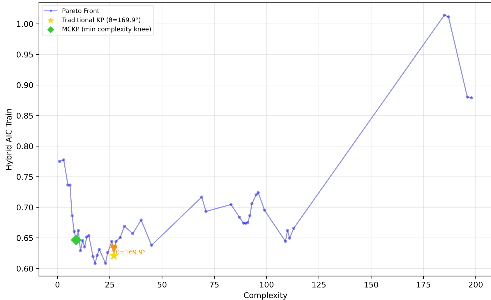
192_vineyard - Run 1 - SVP - Hybrid AIC Train \lambda_1=0.70, \lambda_2=0.70, \lambda_3=0.90 | Difficulty: 0.27 | Method: mckp
