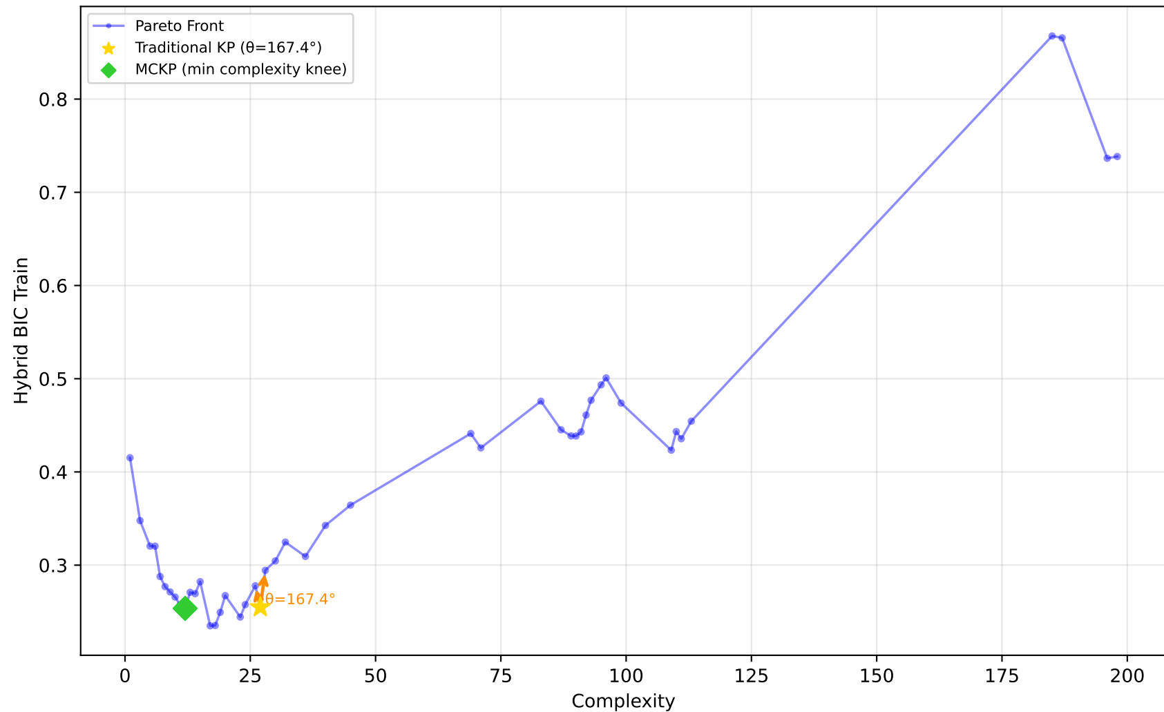
192_vineyard - Run 1 - SVP - Hybrid BIC Train \lambda_1=0.00, \lambda_2=1.00, \lambda_3=1.00 | Difficulty: 0.27 | Method: mckp
