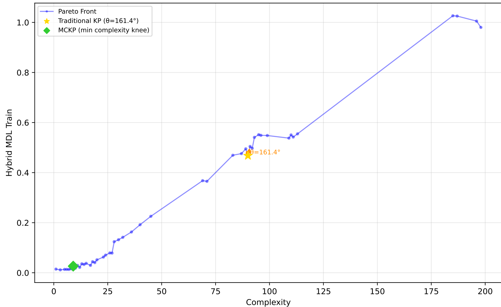
192_vineyard - Run 1 - SVP - Hybrid MDL Train \lambda_1=0.00, \lambda_2=1.00, \lambda_3=1.00 | Difficulty: 0.27 | Method: mckp
