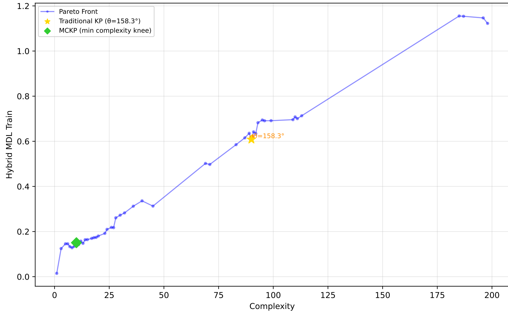
192_vineyard - Run 1 - SVP - Hybrid MDL Train \lambda_1=0.70, \lambda_2=0.70, \lambda_3=0.90 | Difficulty: 0.27 | Method: mckp
