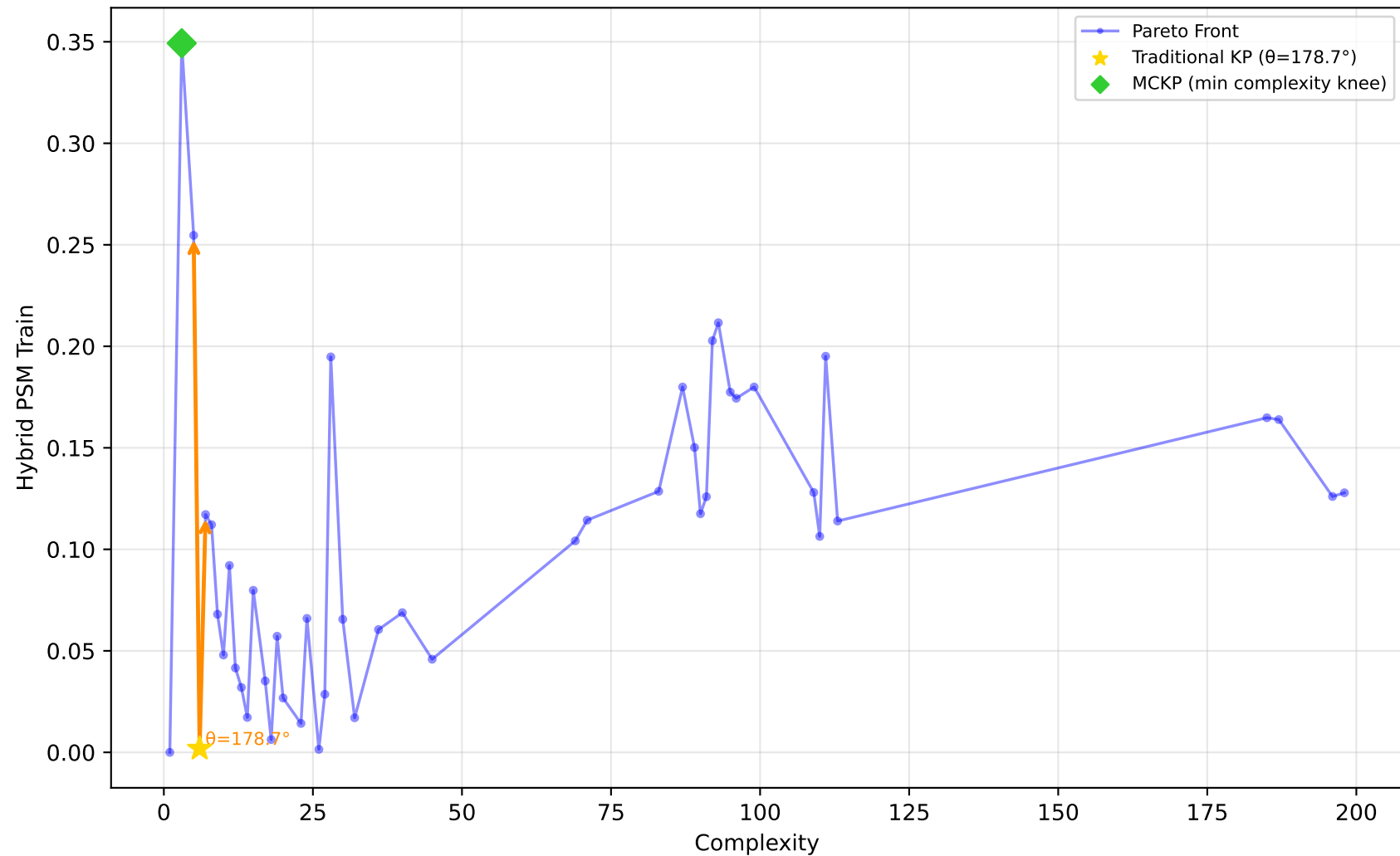
192_vineyard - Run 1 - SVP - Hybrid PSM Train \lambda_1=0.00, \lambda_2=1.00, \lambda_3=1.00 | Difficulty: 0.27 | Method: mckp
