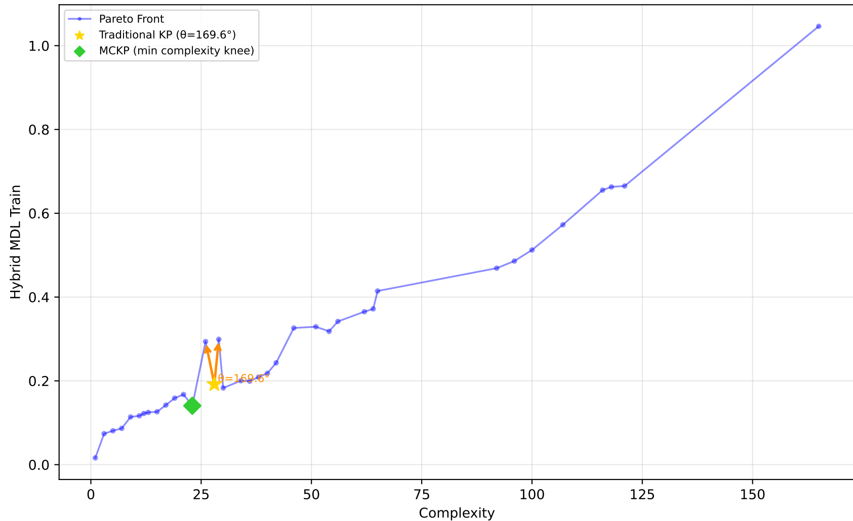
192_vineyard - Run 20 - MVP - Hybrid MDL Train \lambda_1=0.40, \bar{\lambda}_2=0.00, \lambda_3=1.00 | Difficulty: 0.44 | Method: mckp
