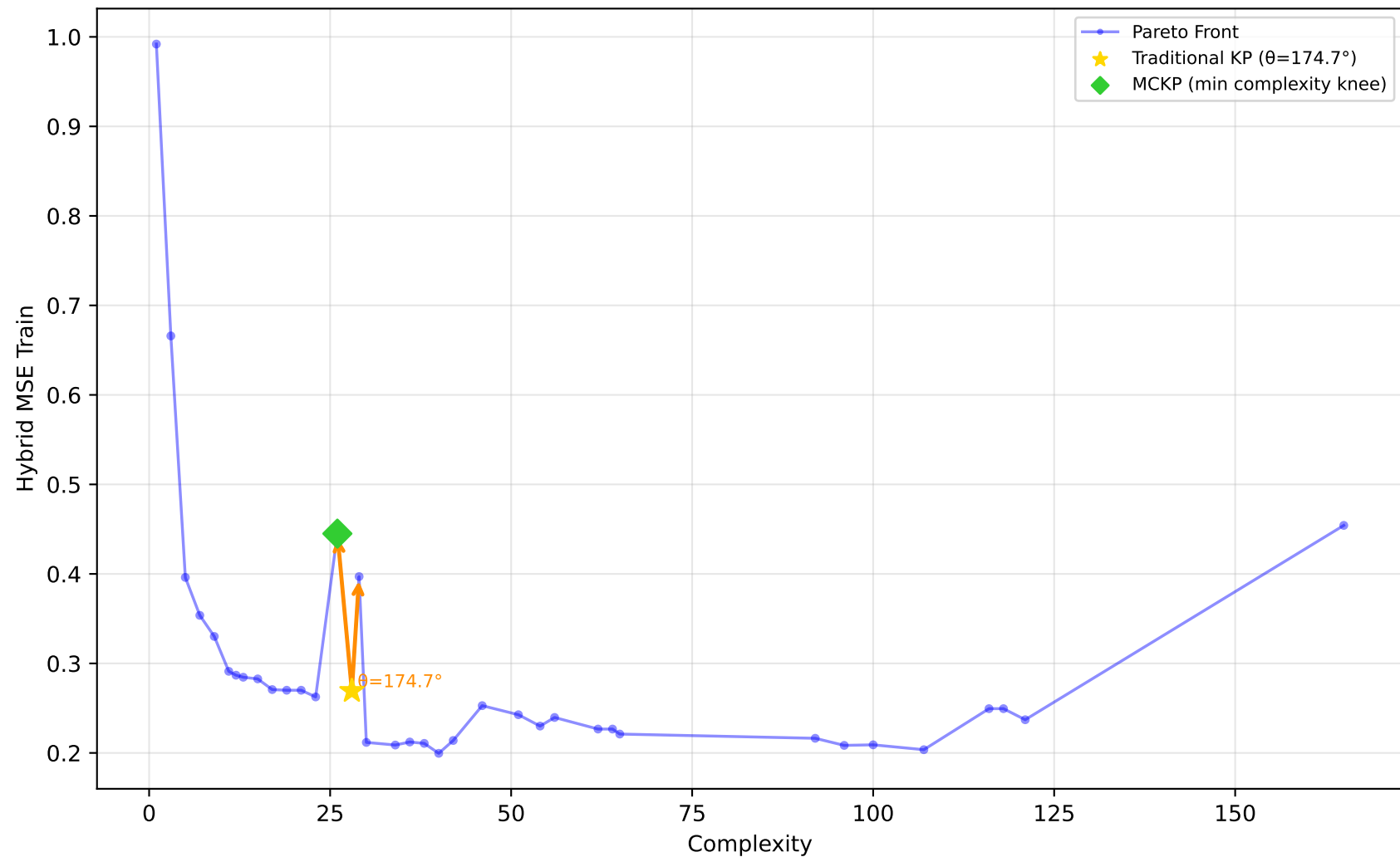
192_vineyard - Run 20 - MVP - Hybrid MSE Train \lambda_1=0.00, \bar{\lambda}_2=0.30, \lambda_3=1.00 | Difficulty: 0.44 | Method: mckp
