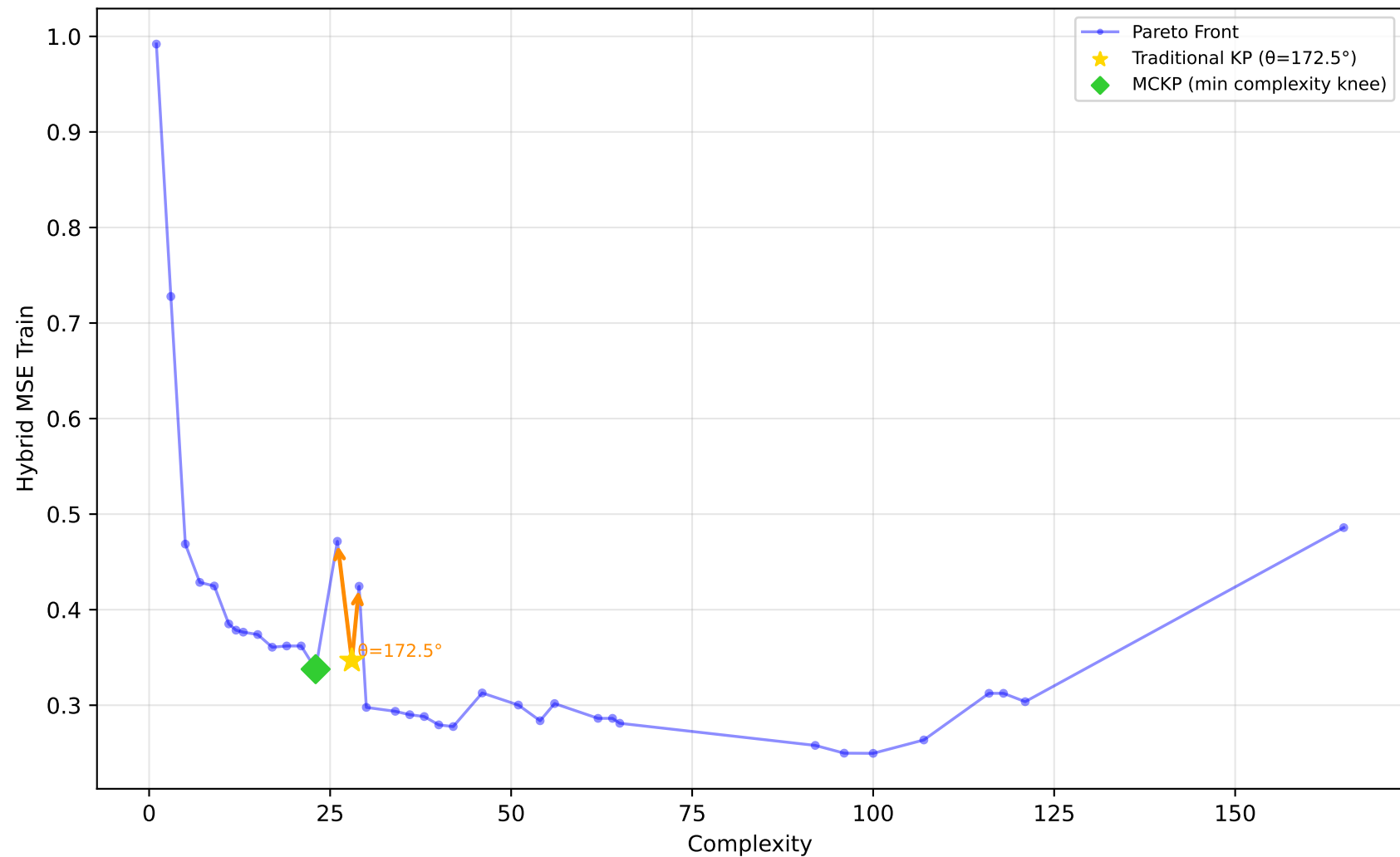
192_vineyard - Run 20 - MVP - Hybrid MSE Train \lambda_1=0.40, \bar{\lambda}_2=0.00, \lambda_3=1.00 | Difficulty: 0.44 | Method: mckp
