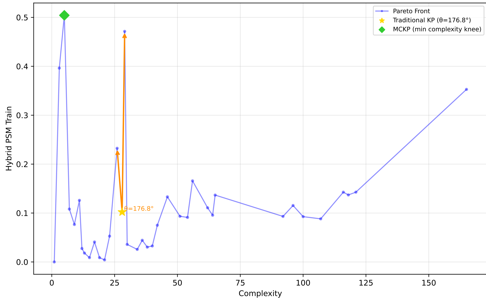
192_vineyard - Run 20 - MVP - Hybrid PSM Train \lambda_1=0.00, \lambda_2=0.30, \lambda_3=1.00 | Difficulty: 0.44 | Method: mckp
