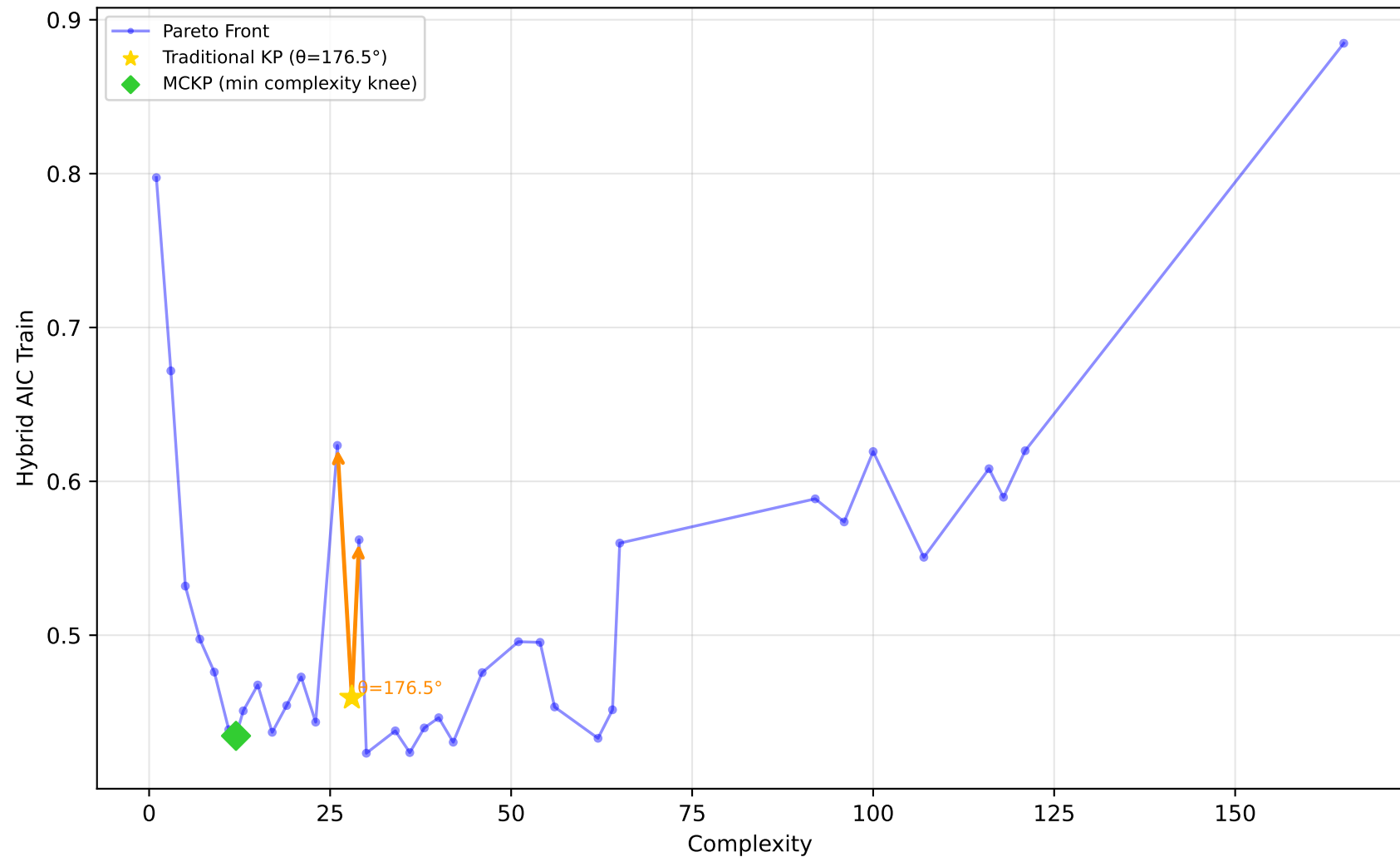
192_vineyard - Run 20 - SVP - Hybrid AIC Train \lambda_1=0.00, \lambda_2=1.00, \lambda_3=1.00 | Difficulty: 0.44 | Method: mckp
