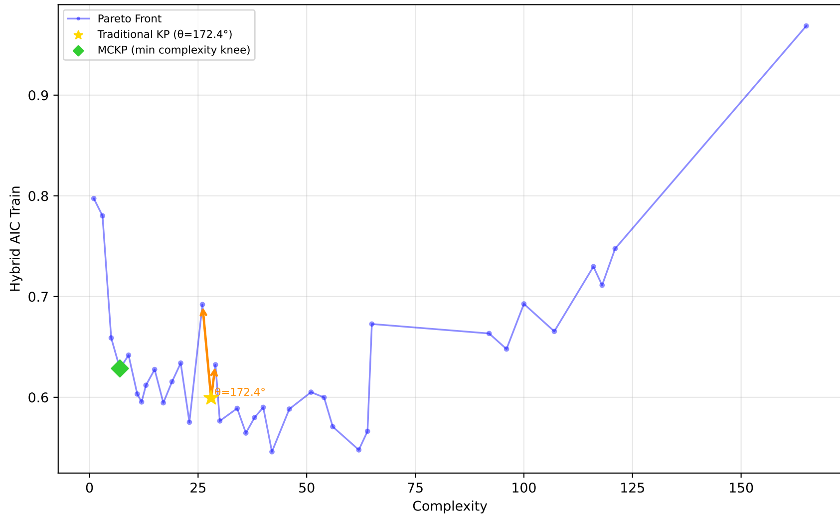
192_vineyard - Run 20 - SVP - Hybrid AIC Train \lambda_1=0.70, \lambda_2=0.70, \lambda_3=0.90 | Difficulty: 0.44 | Method: mckp
