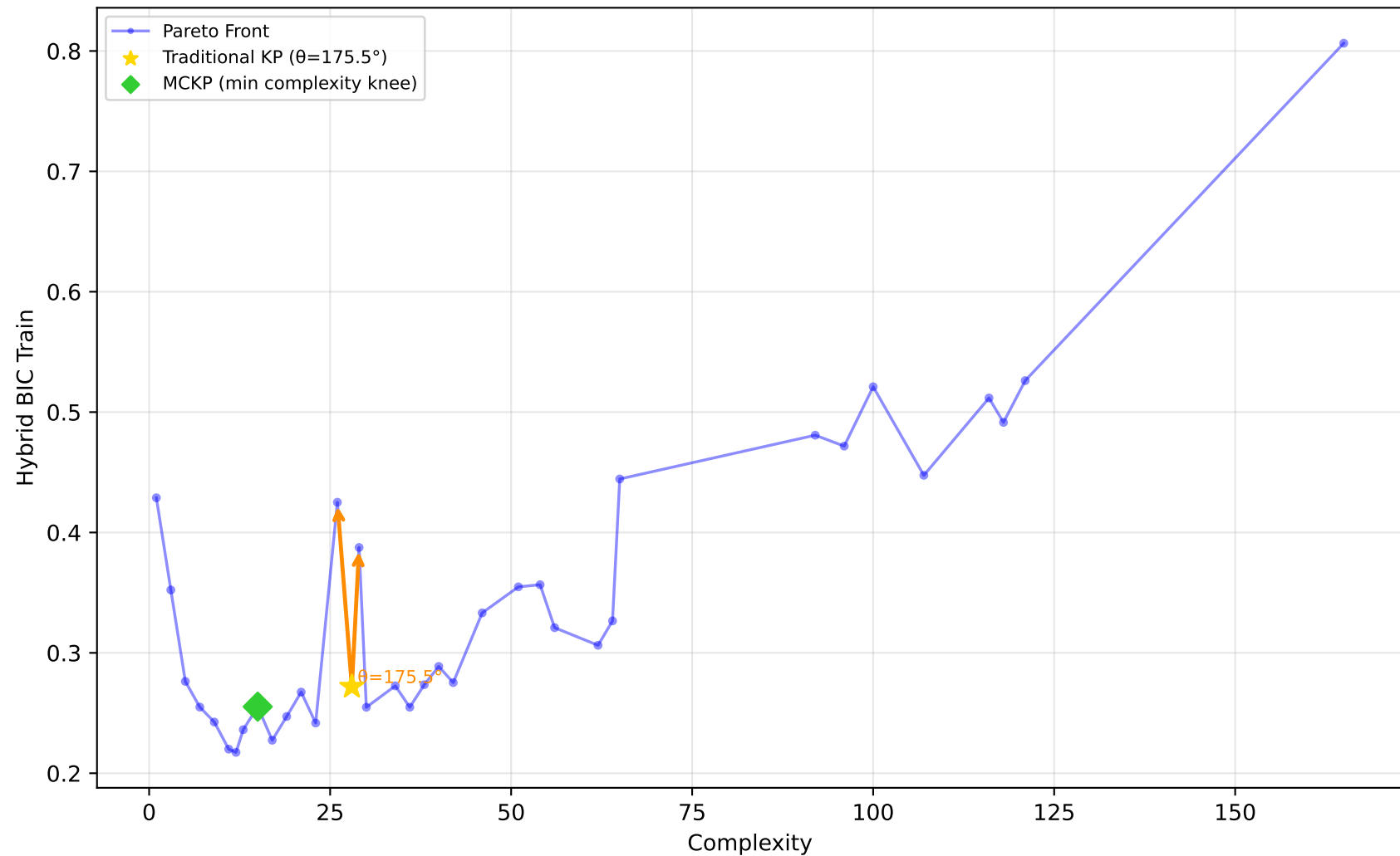
192_vineyard - Run 20 - SVP - Hybrid BIC Train \lambda_1=0.00, \lambda_2=1.00, \lambda_3=1.00 | Difficulty: 0.44 | Method: mckp
