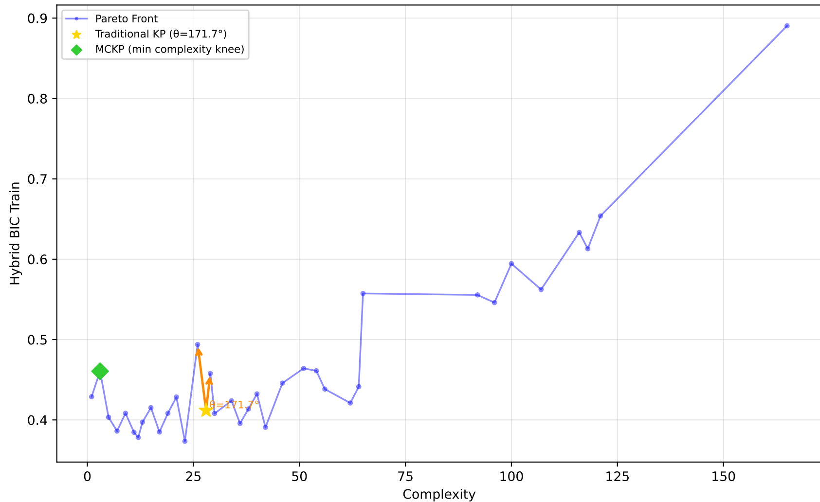
192_vineyard - Run 20 - SVP - Hybrid BIC Train \lambda_1=0.70, \lambda_2=0.70, \lambda_3=0.90 | Difficulty: 0.44 | Method: mckp
