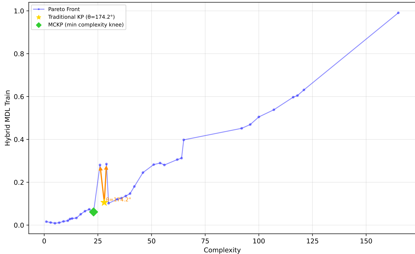
192_vineyard - Run 20 - SVP - Hybrid MDL Train \lambda_1=0.00, \lambda_2=1.00, \lambda_3=1.00 | Difficulty: 0.44 | Method: mckp
