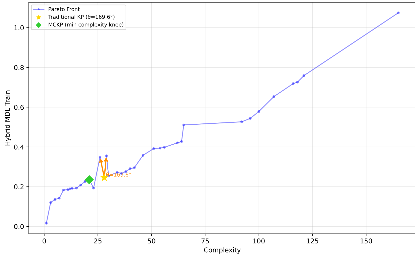
192_vineyard - Run 20 - SVP - Hybrid MDL Train \lambda_1=0.70, \bar{\lambda}_2=0.70, \lambda_3=0.90 | Difficulty: 0.44 | Method: mckp
