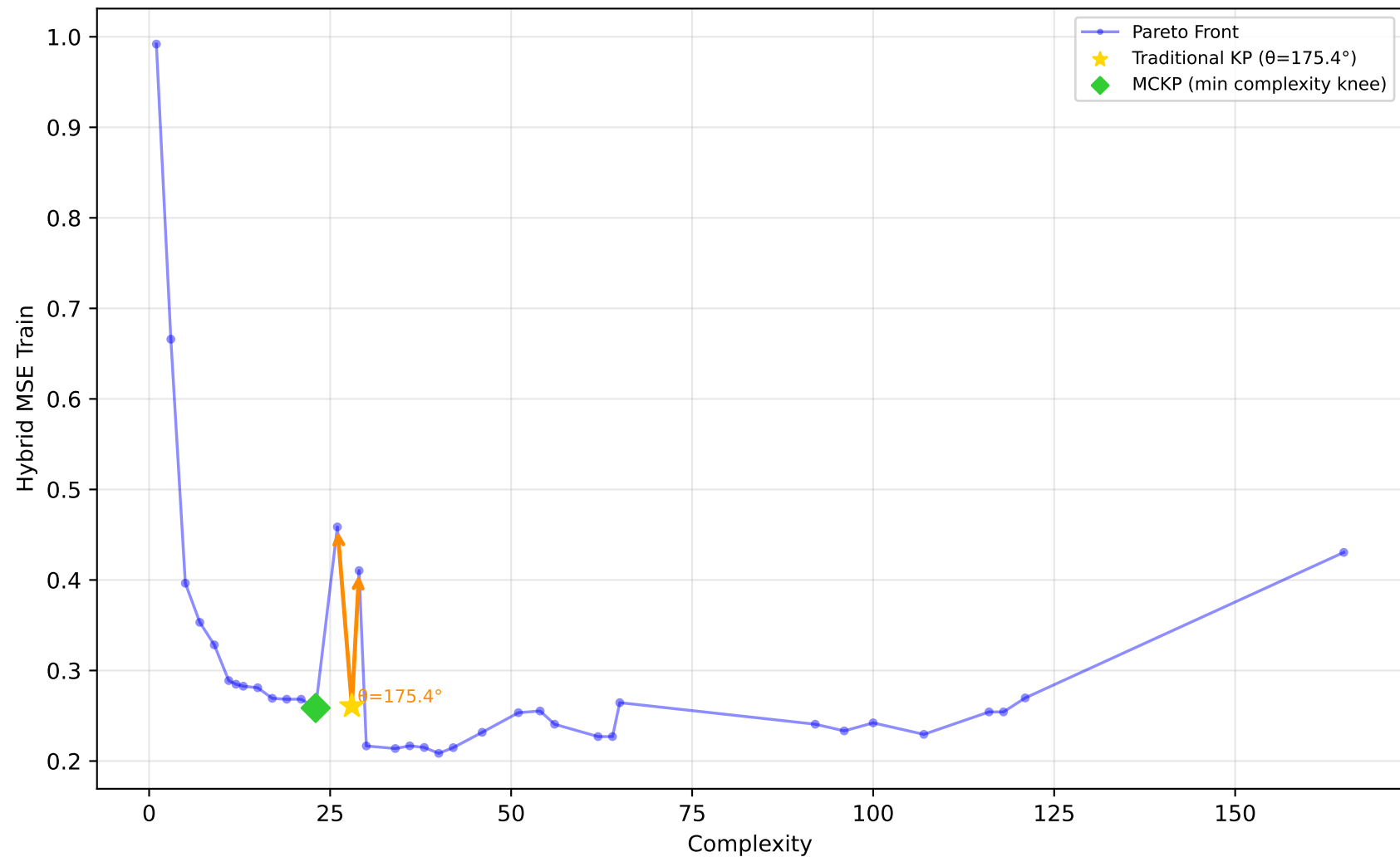
192_vineyard - Run 20 - SVP - Hybrid MSE Train \lambda_1=0.00, \lambda_2=1.00, \lambda_3=1.00 | Difficulty: 0.44 | Method: mckp
