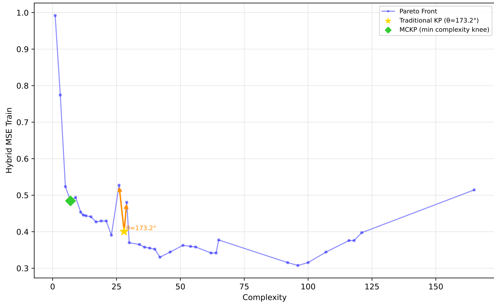
192_vineyard - Run 20 - SVP - Hybrid MSE Train \lambda_1=0.70, \bar{\lambda}_2=0.70, \lambda_3=0.90 | Difficulty: 0.44 | Method: mckp
